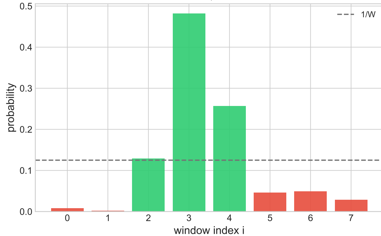
Distribution, P=0.8670
