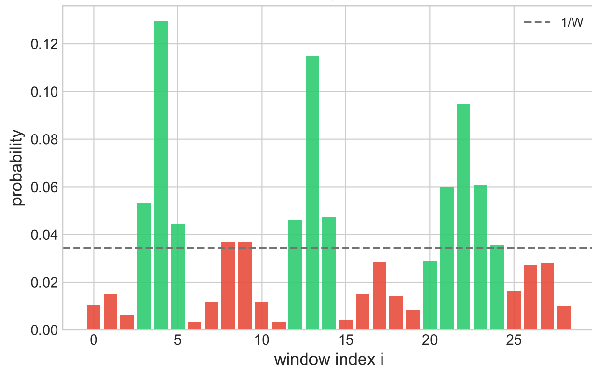
Distribution, P=0.7145
