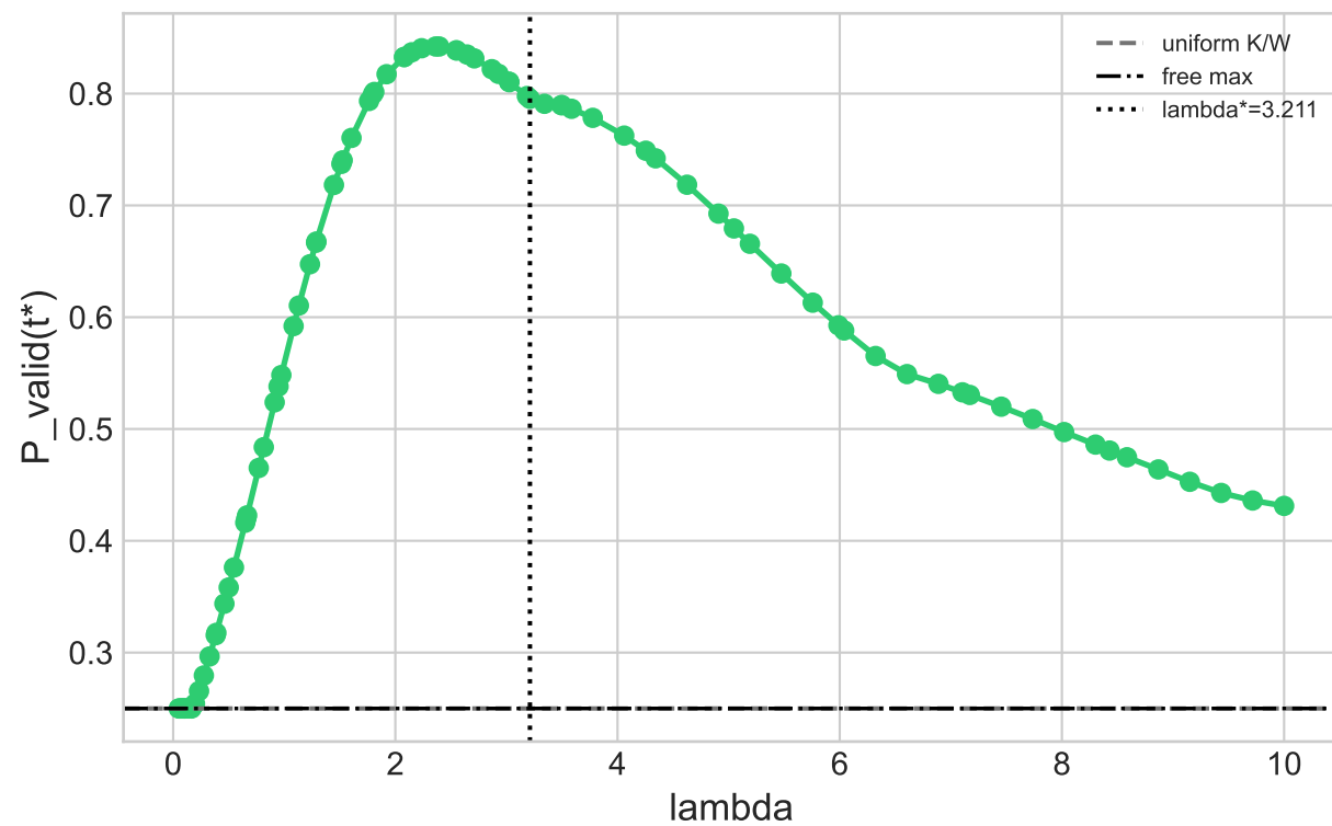
Distribution, P=0.7953
