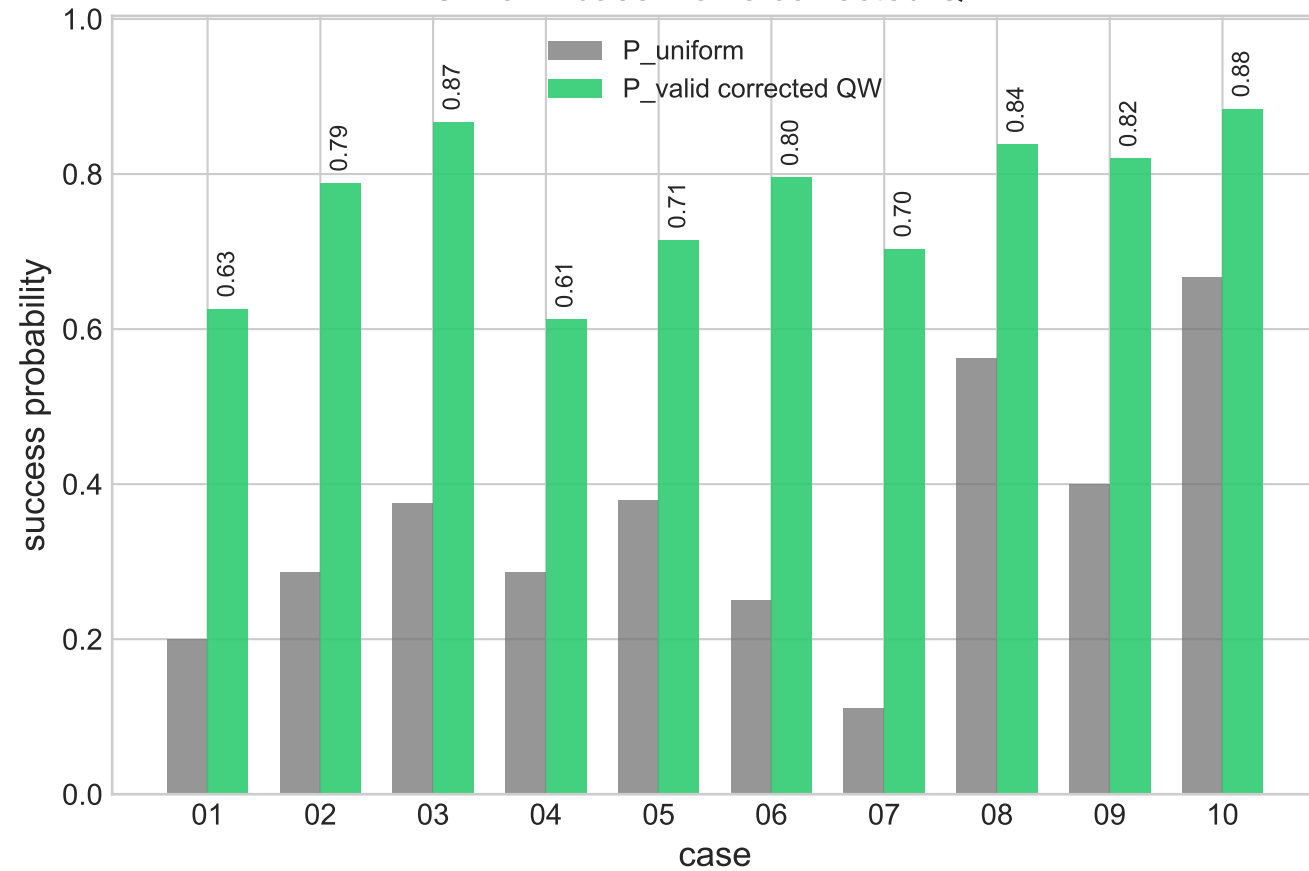
Uniform baseline vs corrected QW
