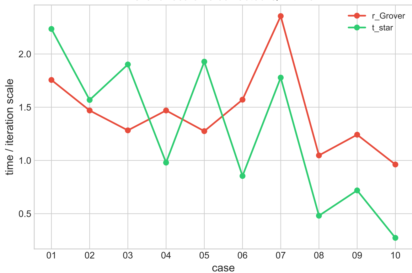
Grover scale vs corrected QW time
