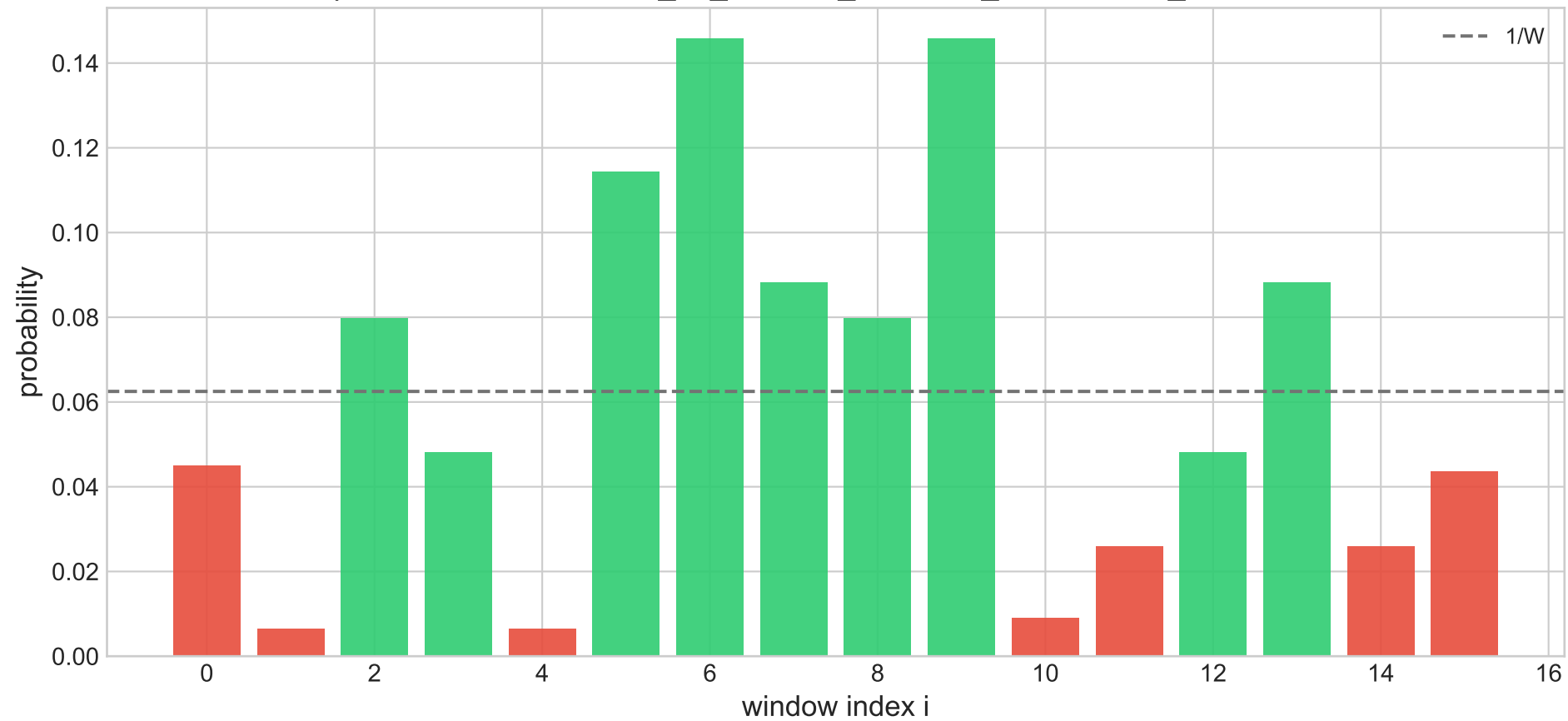
Optimal distribution — 08_2d_medium_clustered_obstacles, P_valid=0.8380
