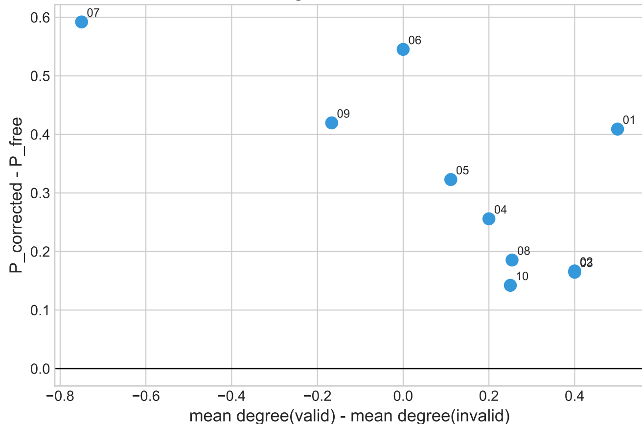
Corrected gain relative to free walk
