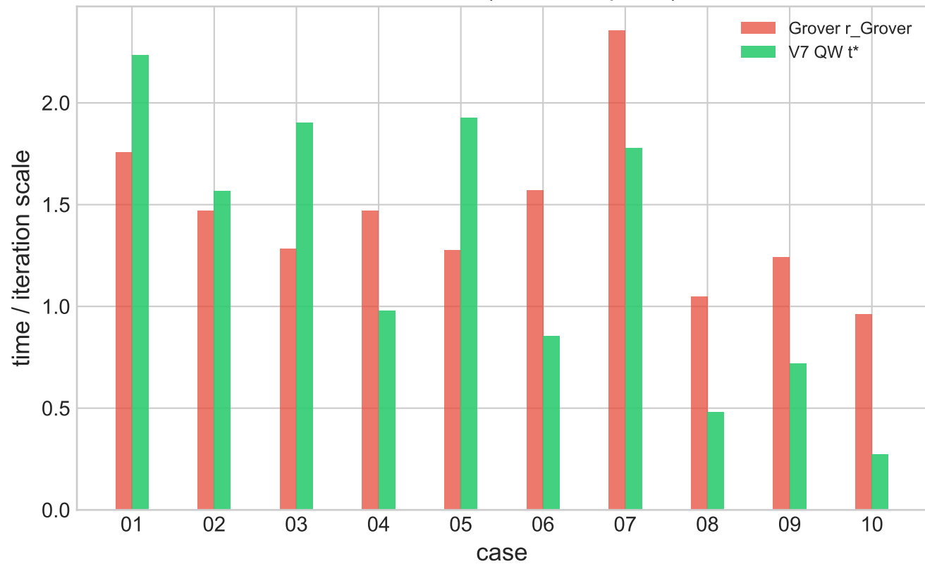
Time face-off (Grover cap ON)
