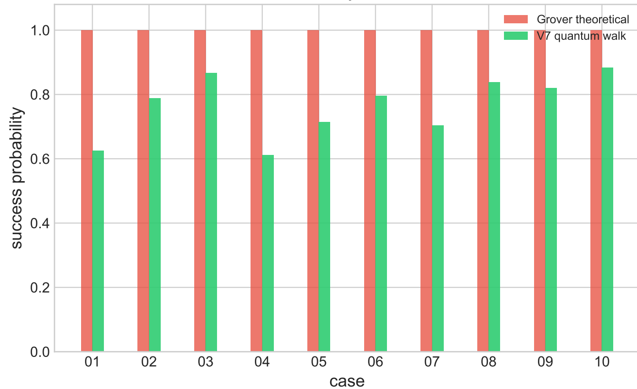
Probability face-off
