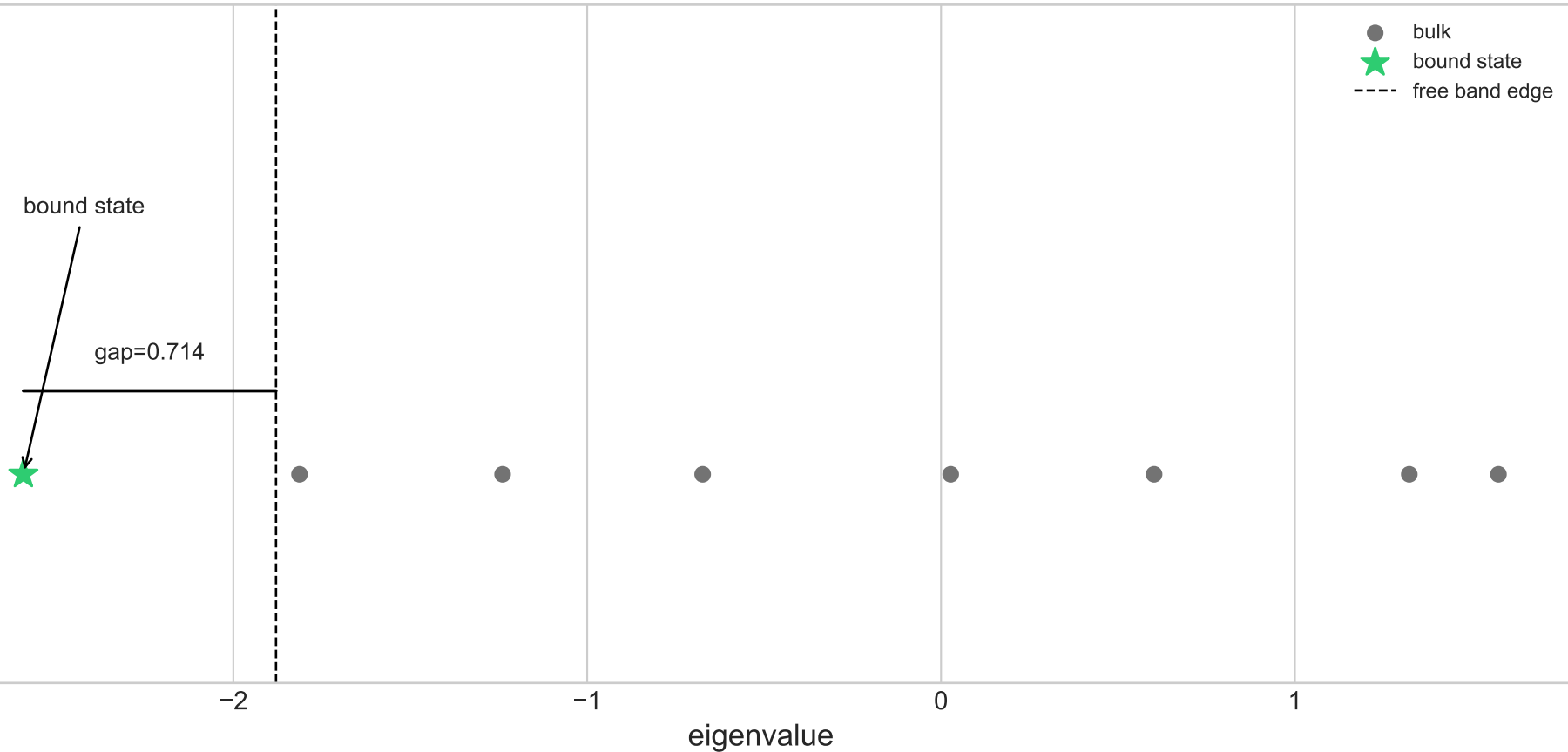
Eigenvalue spectrum — 03_1d_two_free_regions
