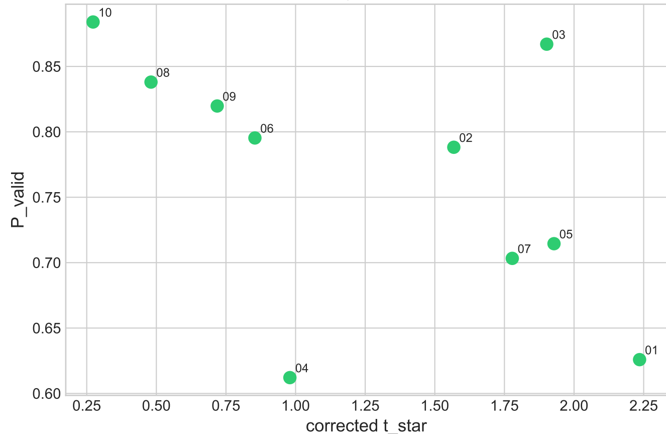
Probability-time tradeoff
