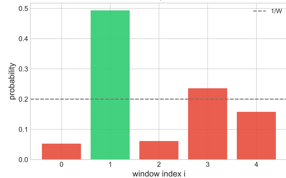
Distribution, P=0.4929
