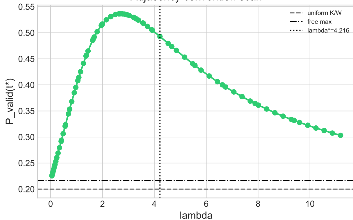
Distribution, P=0.4929
