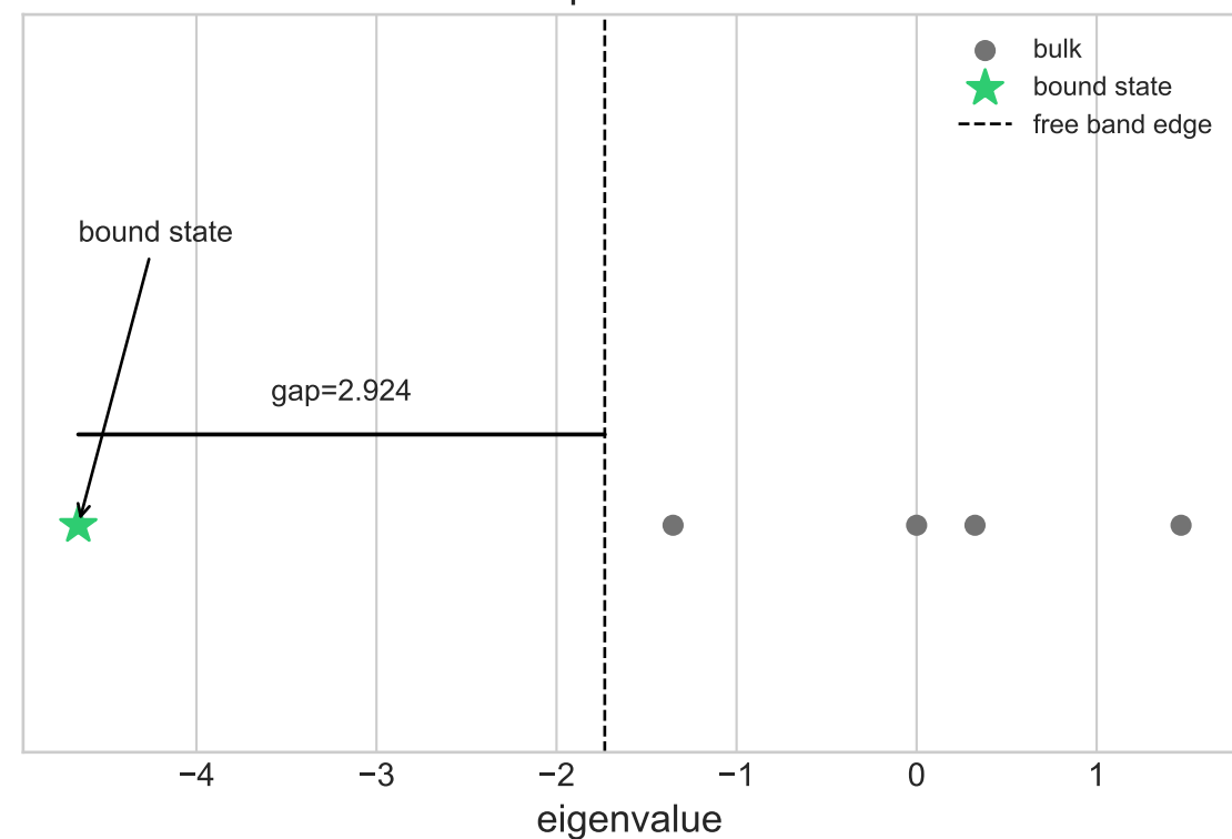
Spectrum
