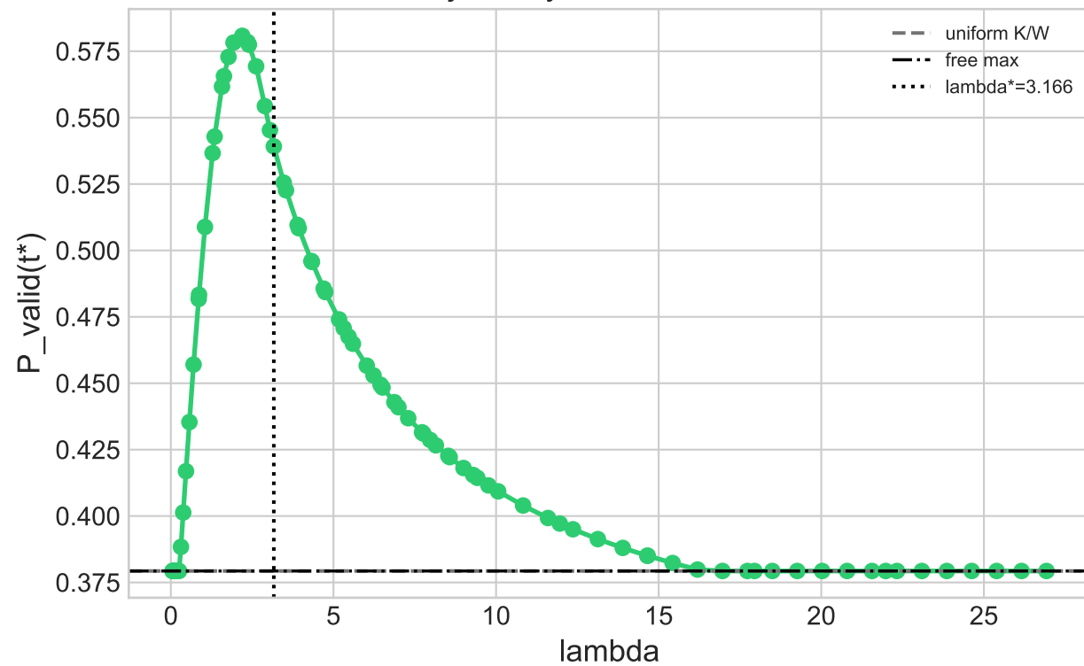
Distribution, P=0.5392
