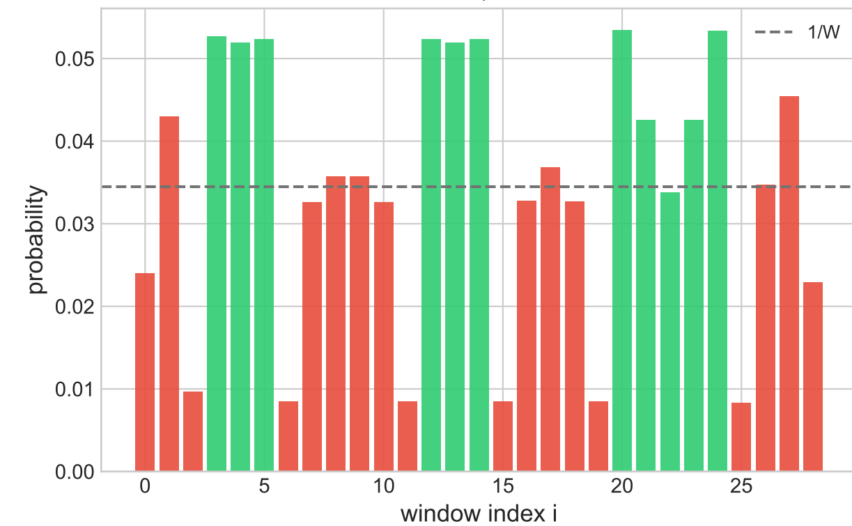
Distribution, P=0.5392
