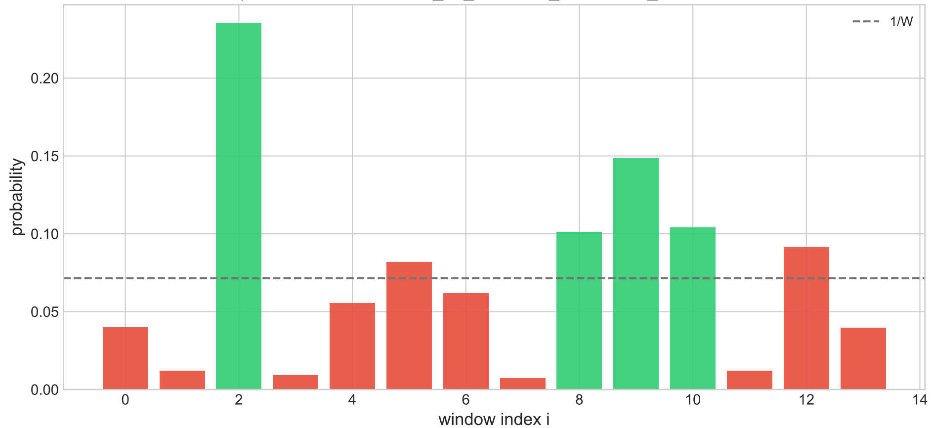
Optimal distribution — 04_1d_clustered_medium, P_valid=0.5892
