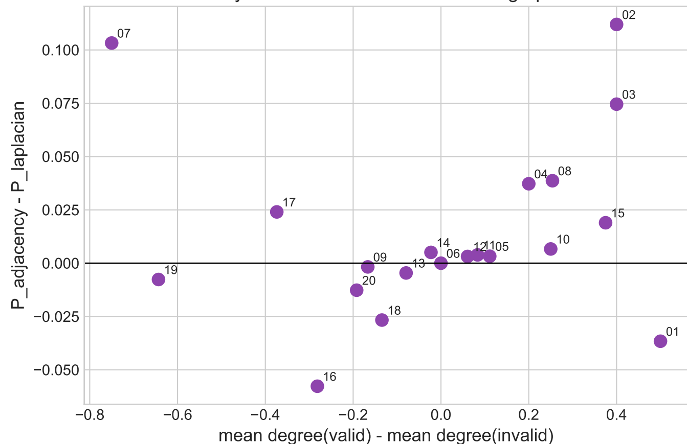
Why the conventions differ on finite graphs
