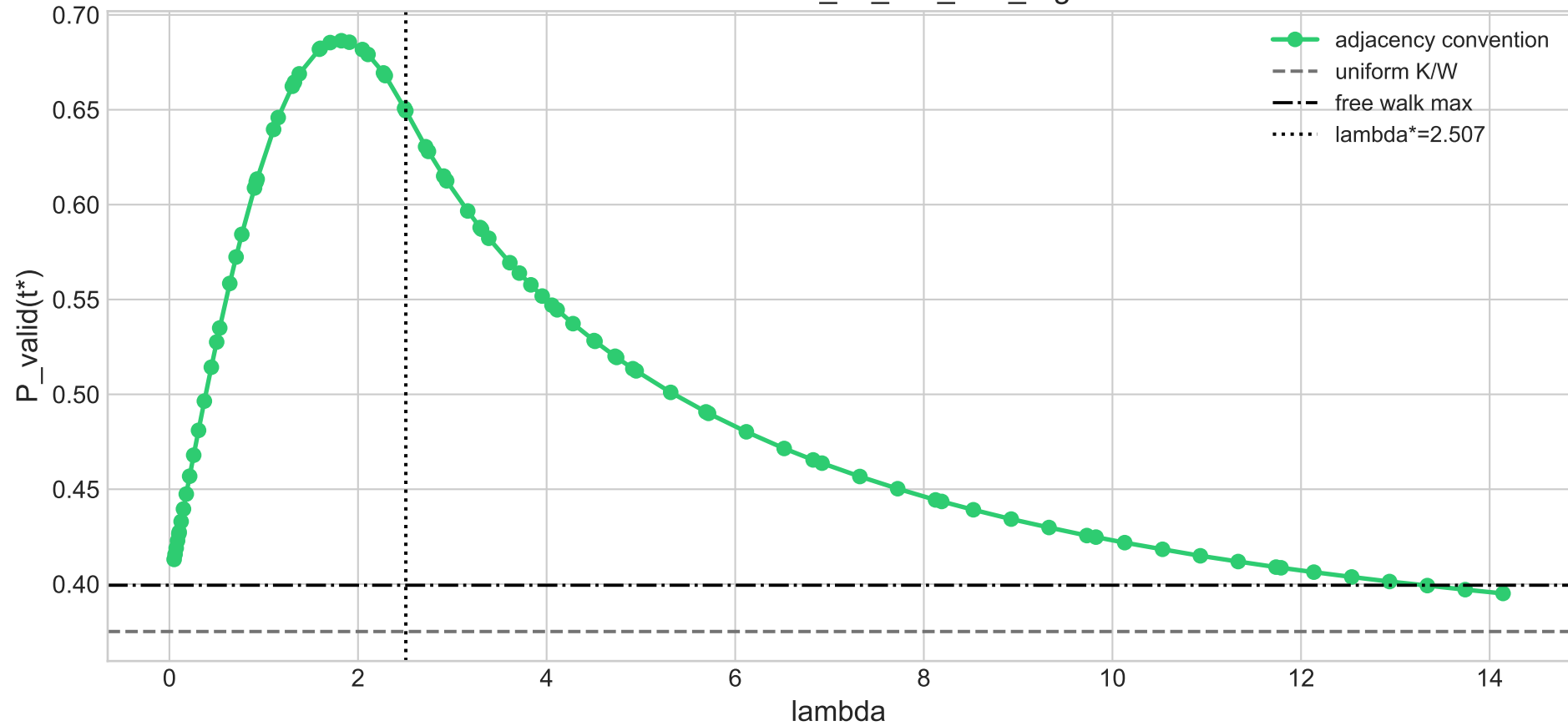
Lambda scan — 03_1d_two_free_regions
