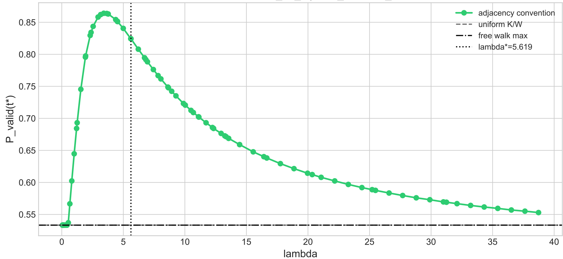
Lambda scan — 20_3d_layered_obstacle_bands
