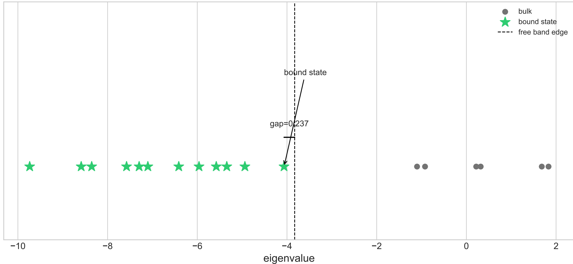
Eigenvalue spectrum — 10_3d_small_clustered_obstacles
