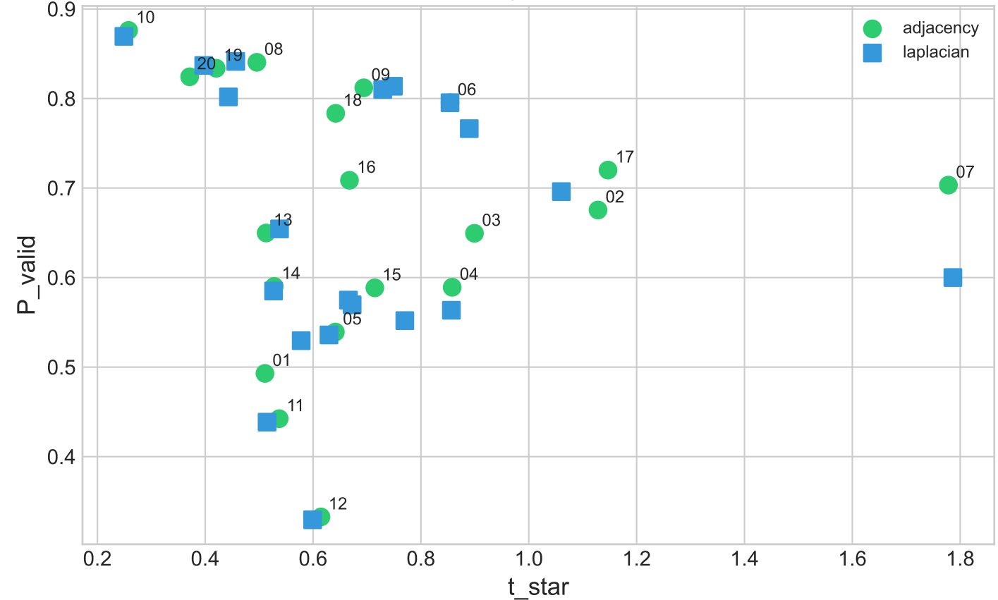
Probability-time tradeoff
