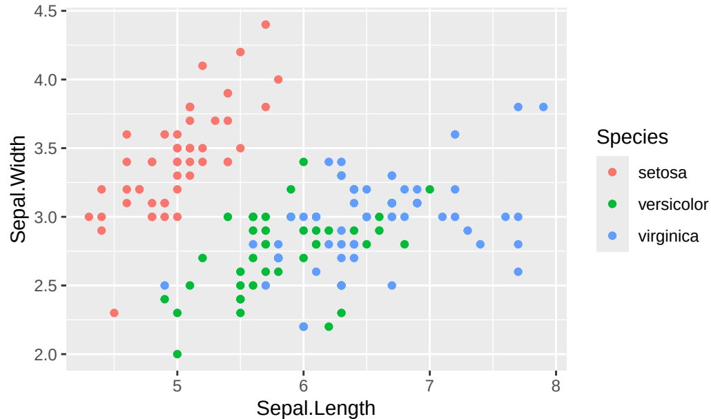
Sepal length and width in the iris dataset
