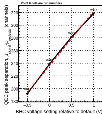
BHC paddle 10
