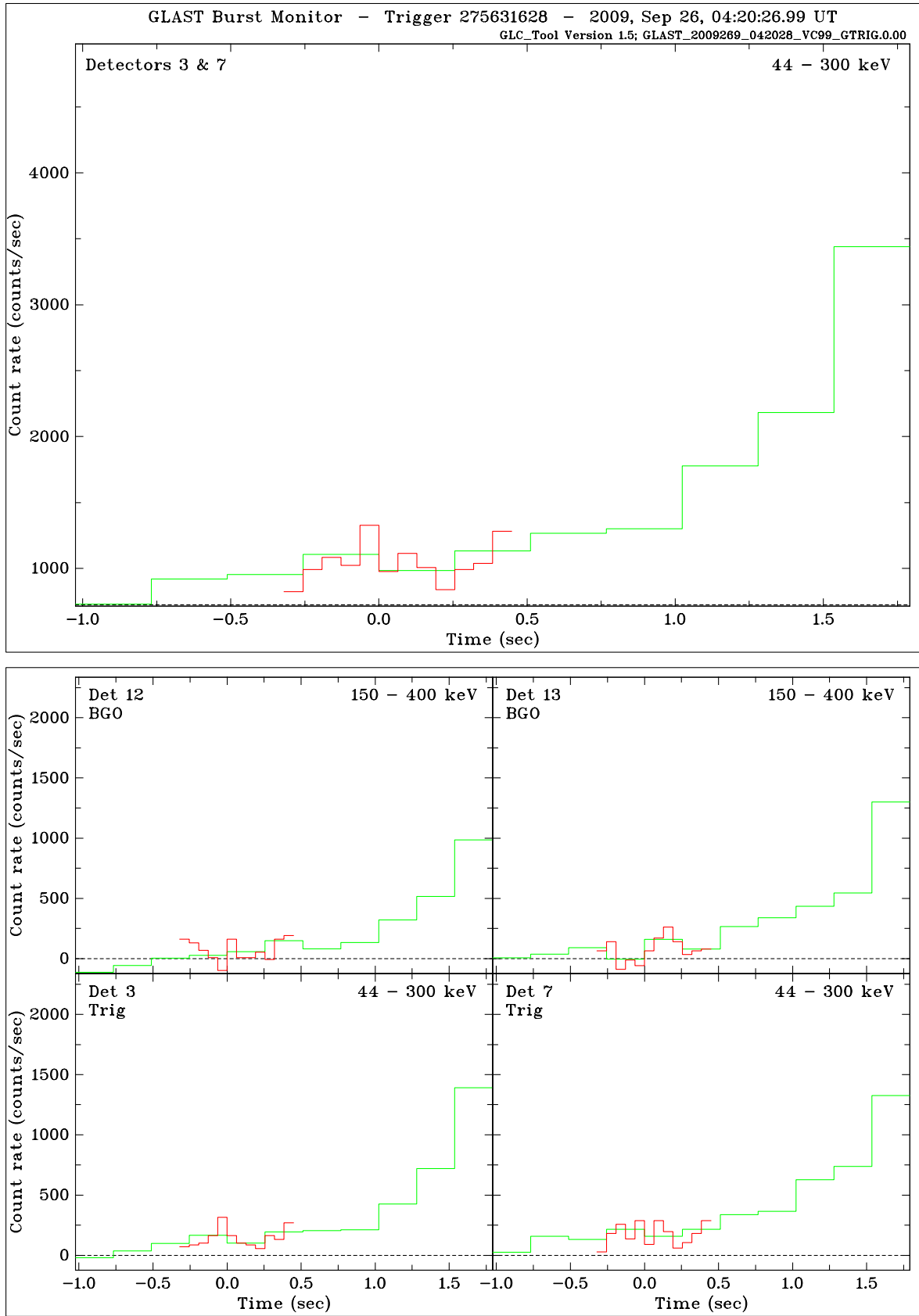
Figure 3: Light curves of the two trigger detectors combined (top); and of the two trigger detectors and two BGO detectors after background subtraction (bottom).
