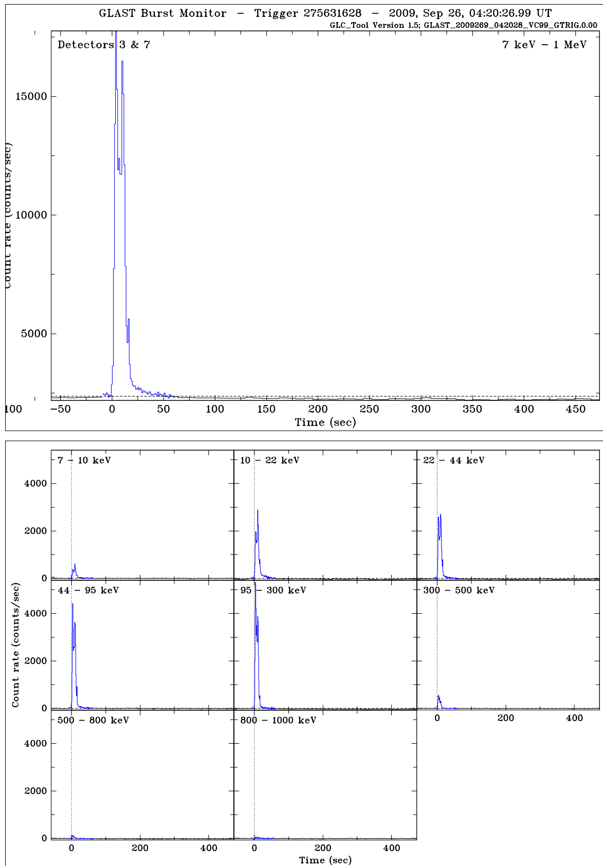
Figure 1: Light curves of the two trigger detectors combined (top); and in the 8 energy channels (bottom).
