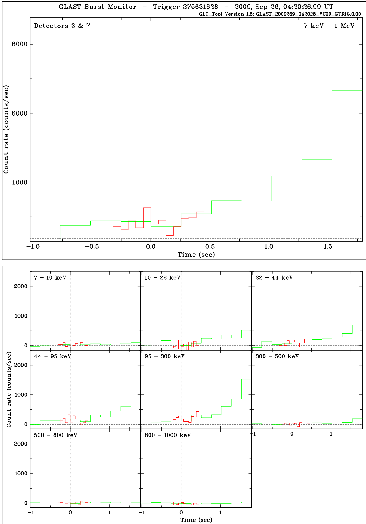
Figure 3: Light curves of the two trigger detectors combined (top); and in the 8 energy channels (bottom).
