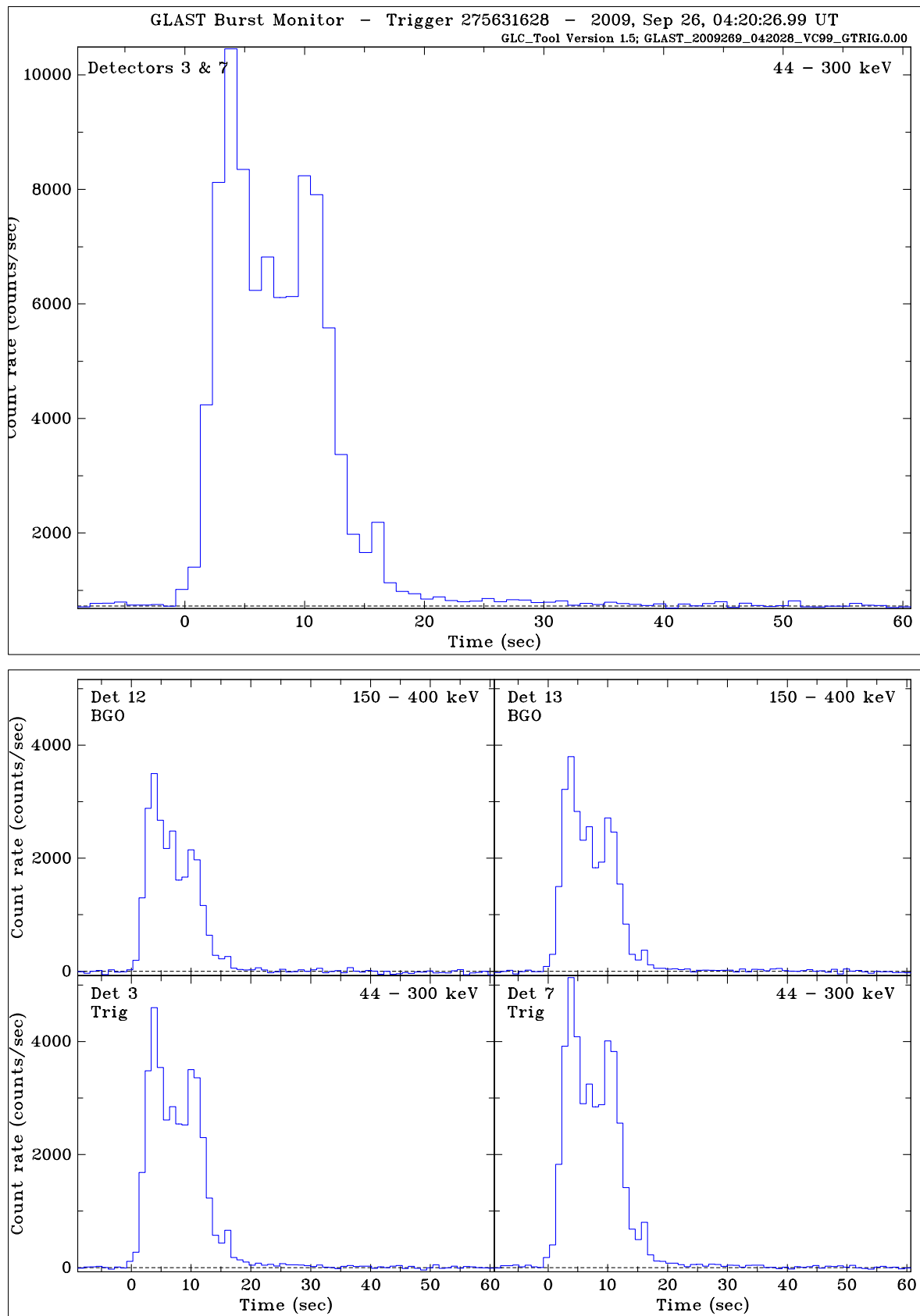
Figure 2: Light curves of the two trigger detectors combined (top); and of the two trigger detectors and two BGO detectors after background subtraction (bottom).
