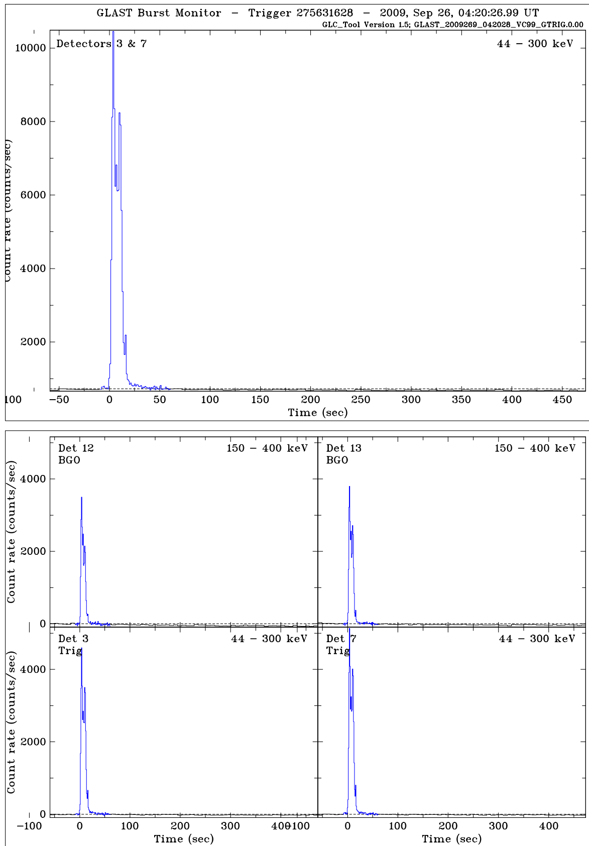
Figure 1: Light curves of the two trigger detectors combined (top); and of the two trigger detectors and two BGO detectors after background subtraction (bottom).
