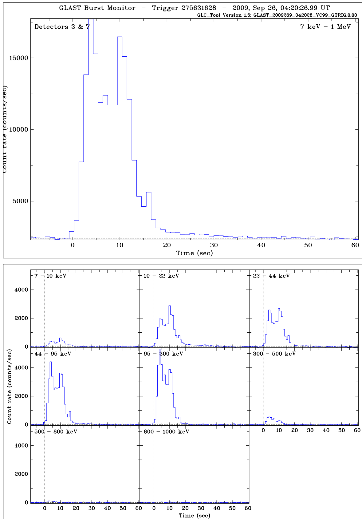
Figure 2: Light curves of the two trigger detectors combined (top); and in the 8 energy channels (bottom).
