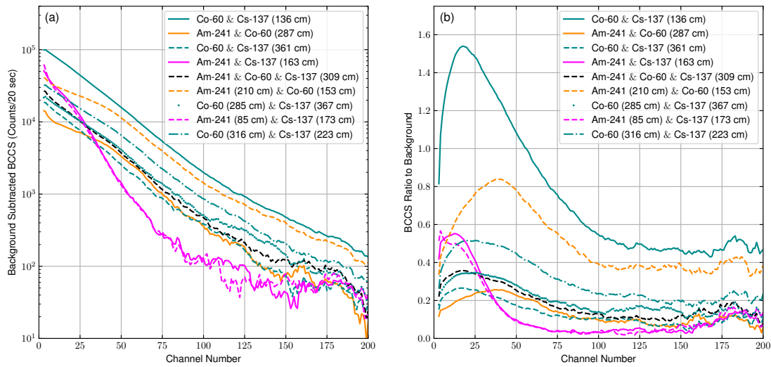
Figure 2. Processed BCCS spectra for mixed-source measurements. (a) Background-subtracted BCCS spectra for nine mixed-source configurations consisting of Am-241, Cs-137, and Co-60 at different source-to-detector distances. Absolute count differences among mixtures are preserved, revealing mixture-dependent cumulative spectral profiles. (b) Background-normalized BCCS spectra for the same configurations. Normalization emphasizes relative deviations from background and enhances the visibility of spectral differences among mixtures, particularly when radionuclides contribute differently across channel regions.
