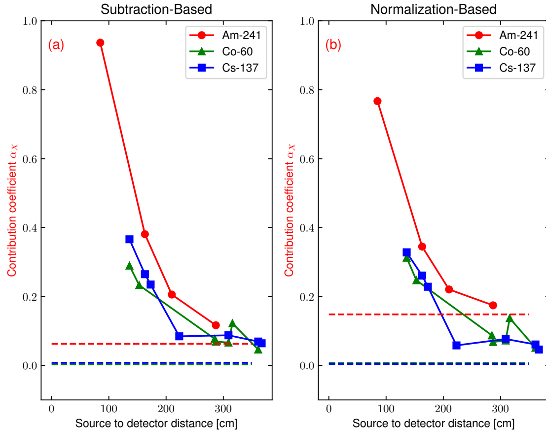
Figure 5. Estimated contribution coefficients \alpha_X for Am-241, Co-60, and Cs-137 as a function of source-to-detector distance. Each coefficient is expressed relative to the corresponding reference measurement of that radionuclide (Table 1) and is therefore not directly comparable between radionuclides. For configurations in which the two sources were placed at different distances, each point is plotted at the distance of the corresponding source. (a) results from the subtraction-based method; (b) results from the normalization-based method. Horizontal dashed lines indicate mean contribution levels estimated from measurements in which the corresponding radionuclide was absent, providing practical background-derived decision thresholds. The inferred contributions decrease with increasing distance and approach the threshold bands under very weak-signal conditions.
