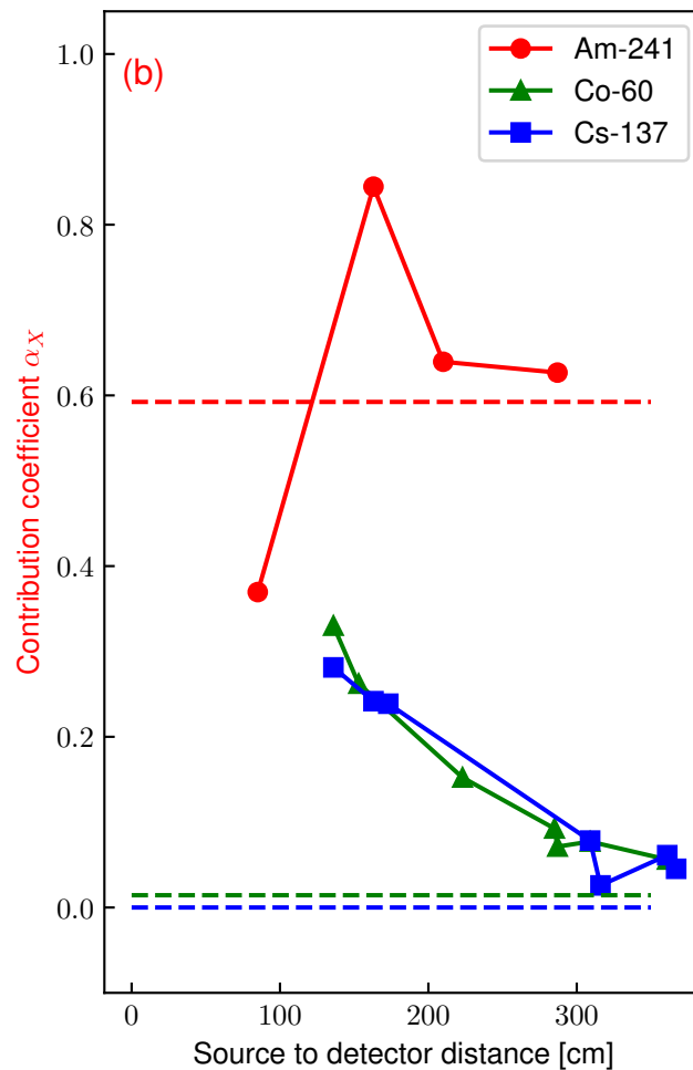
Normalization-Based
