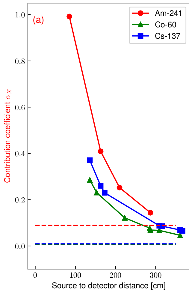
Subtraction-Based
