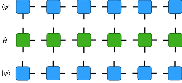
Fig. 2: The expectation value of an operator \hat{H} is shown in tensor diagram notation for a 6-site system. When contracted, this would give \langle\hat{H}\rangle , or the energy E if \hat{H} is the Hamiltonian. The wavefunction on the bottom row alone would be represented as in the text (Eq. 1), which is far more intricate.
