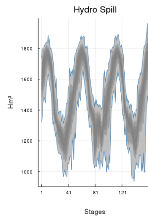
Fig. 7. Hydro Spill (Storage Spillage)
