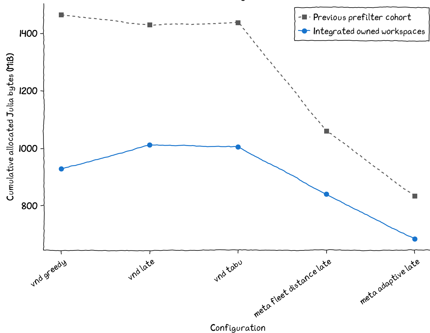
LCIOI: 30-second diagnostic allocations
