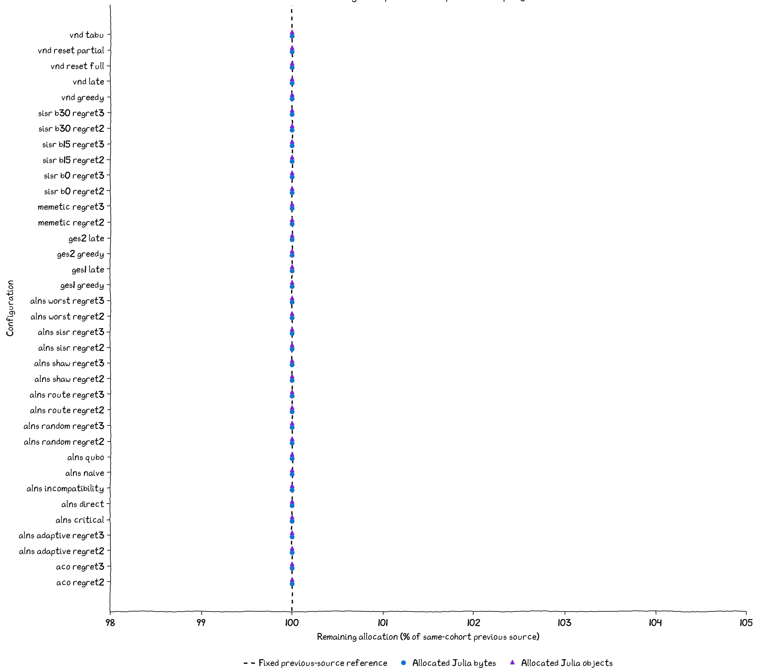
Routing search profiles: bounded private cache capacity
