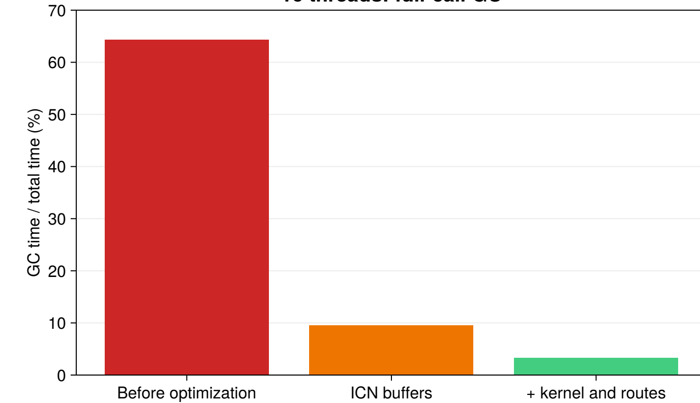
16 threads: full-call GC
