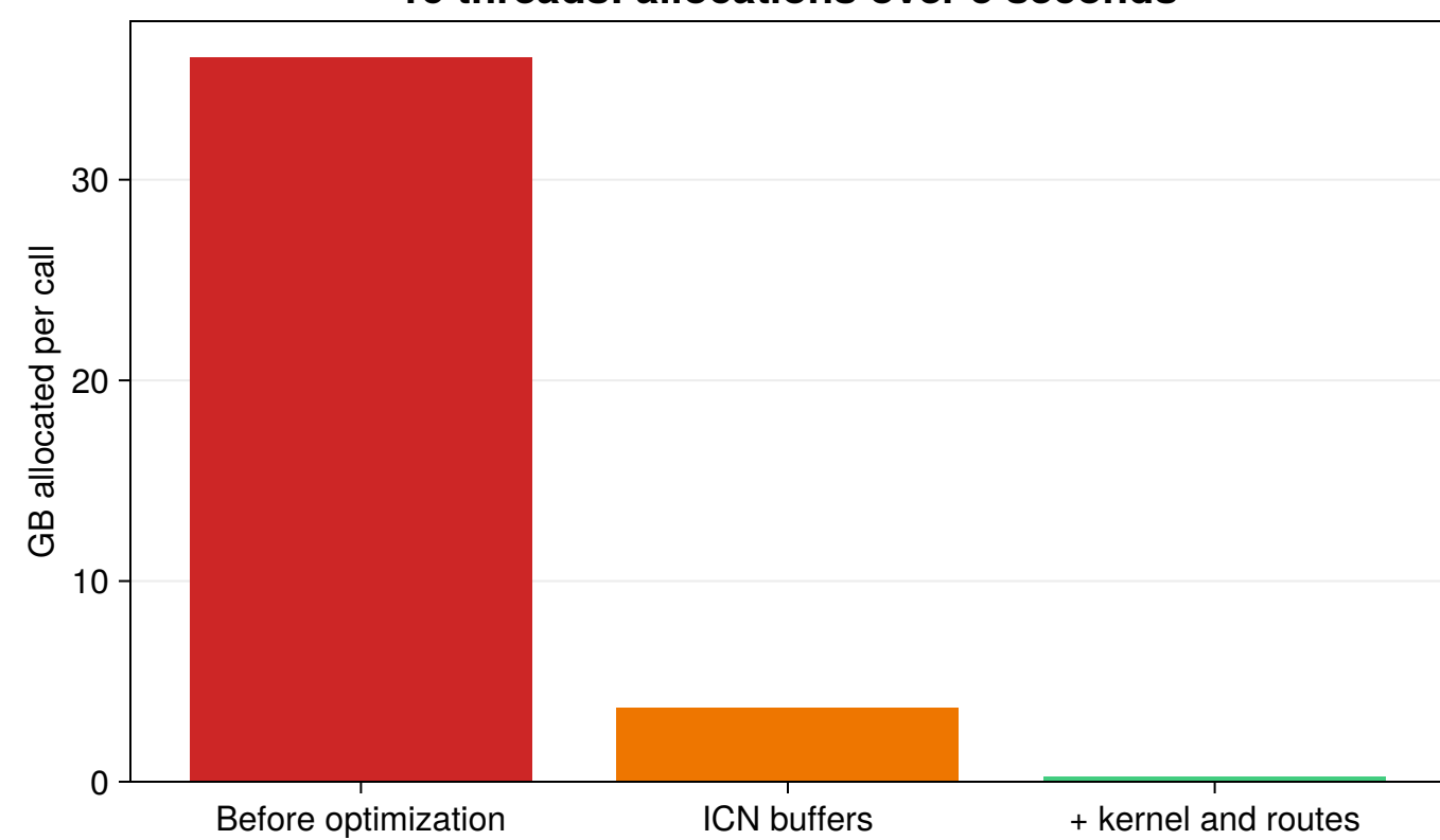
16 threads: allocations over 5 seconds
