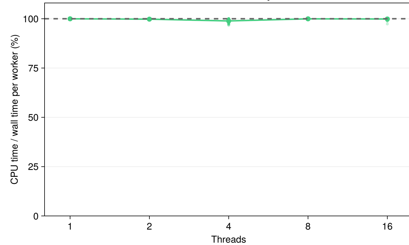
Worker utilization after optimization
