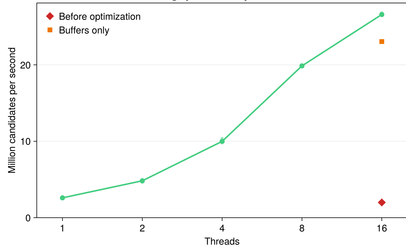
Throughput after optimization
