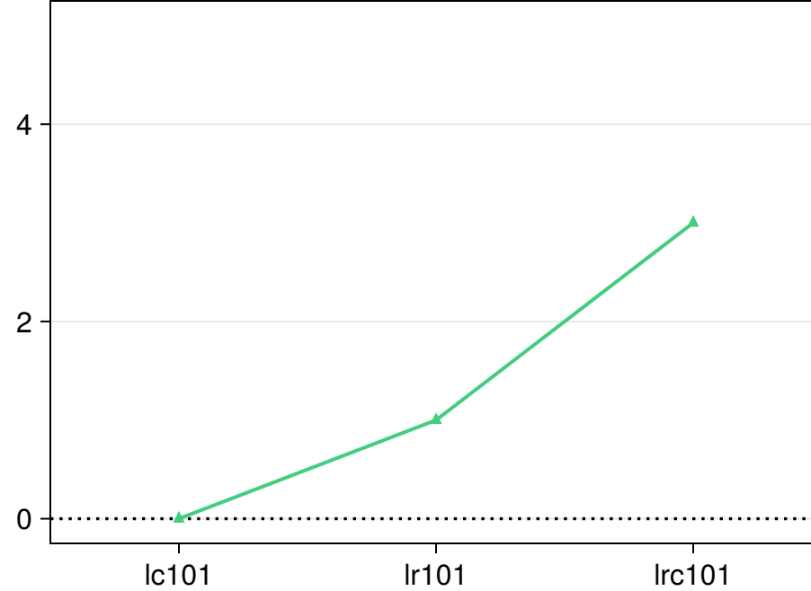
HiGHS portfolio
