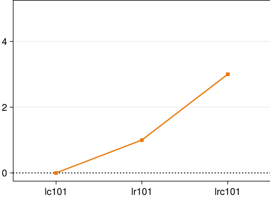
HiGHS native
