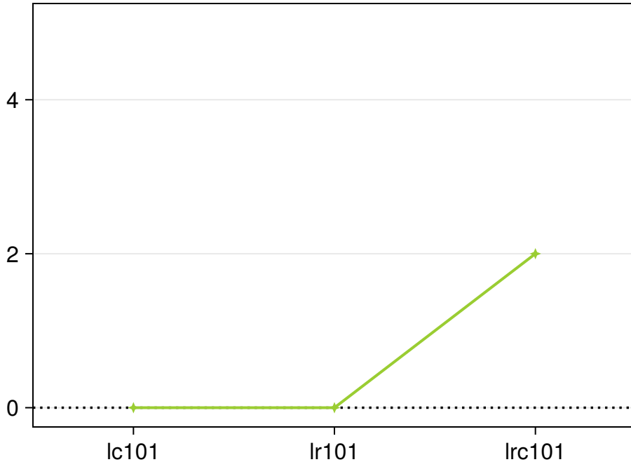
MetaStrategist search-heavy
