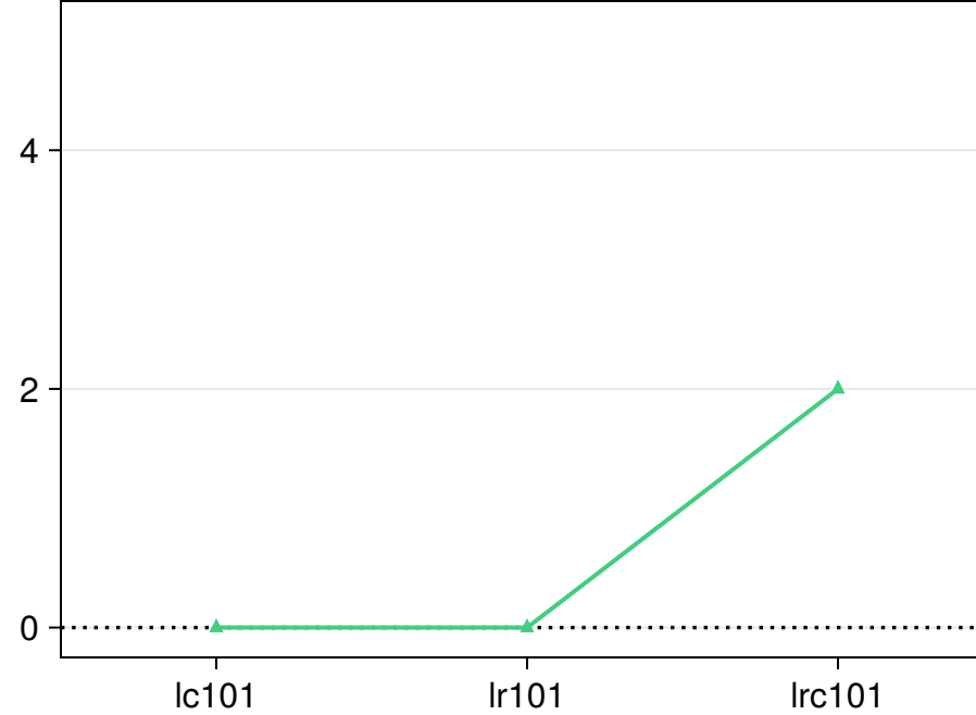
HiGHS portfolio
