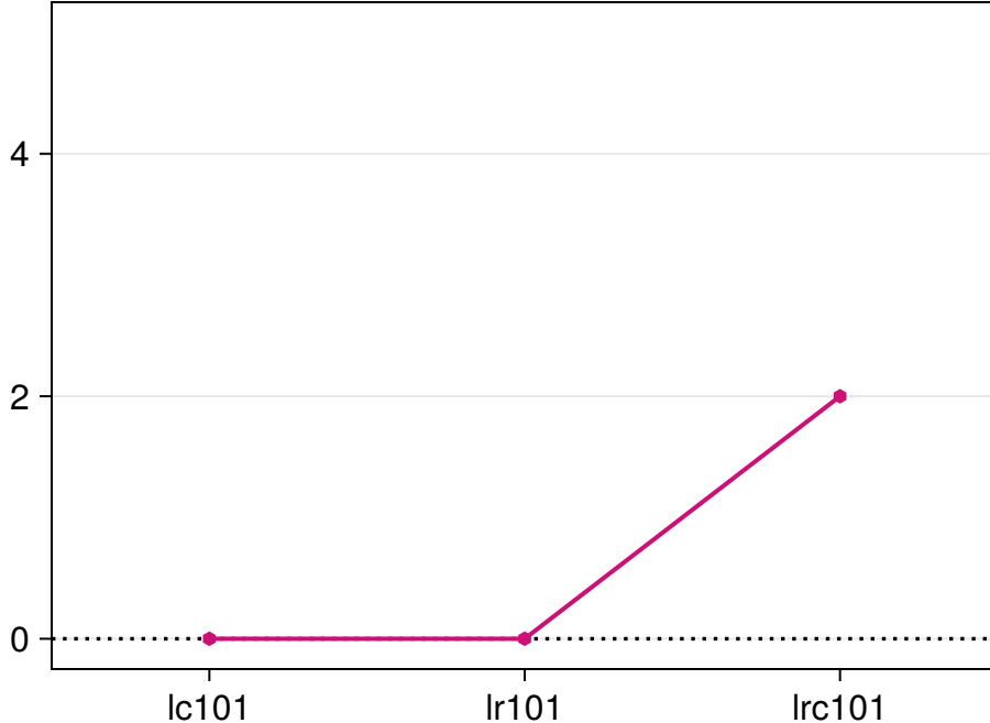
MetaStrategist search-heavy
