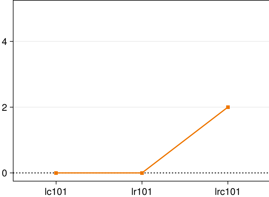
HiGHS native
