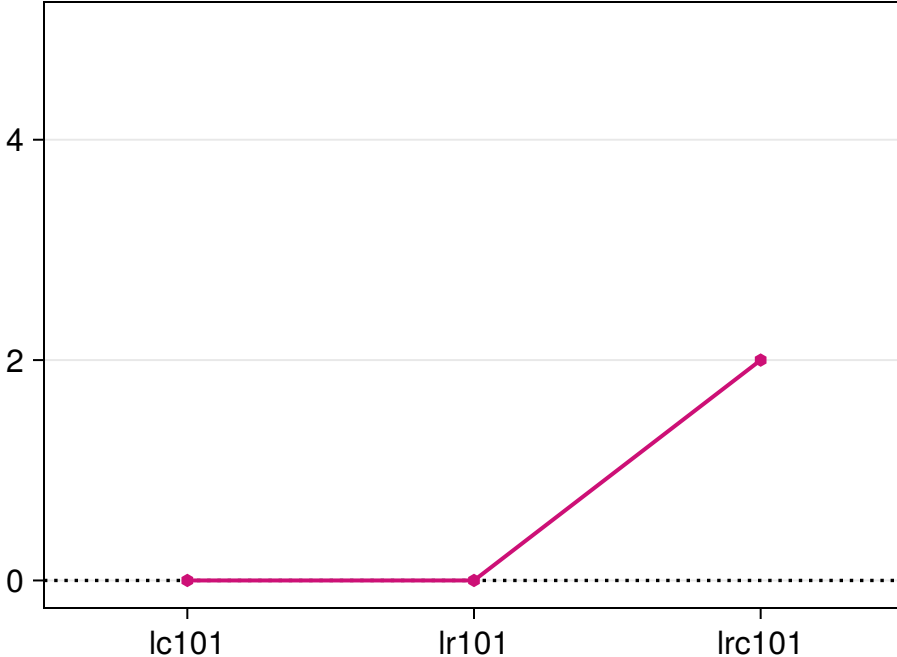
MetaStrategist search-heavy
