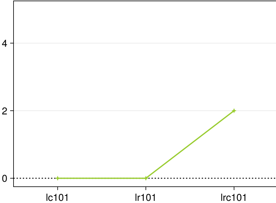
MetaStrategist search-heavy
