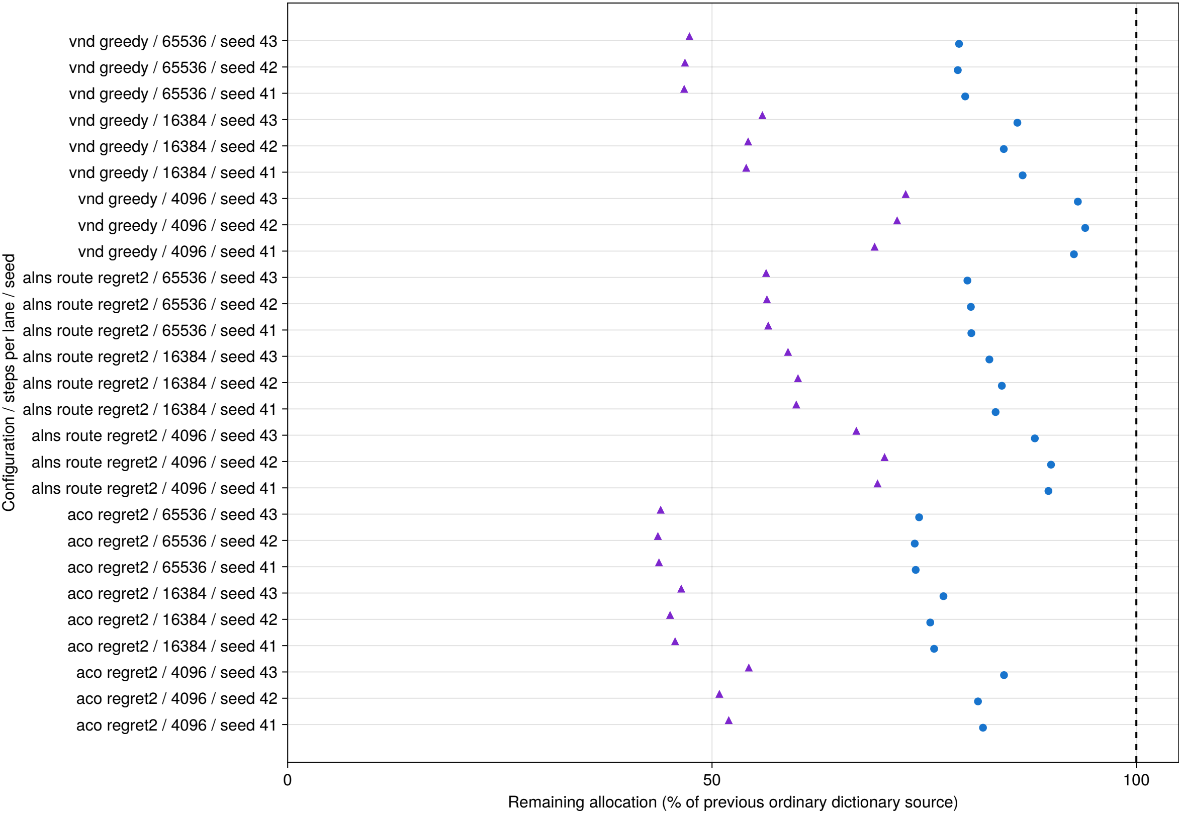
Original LR101: numeric traces at identical search work
