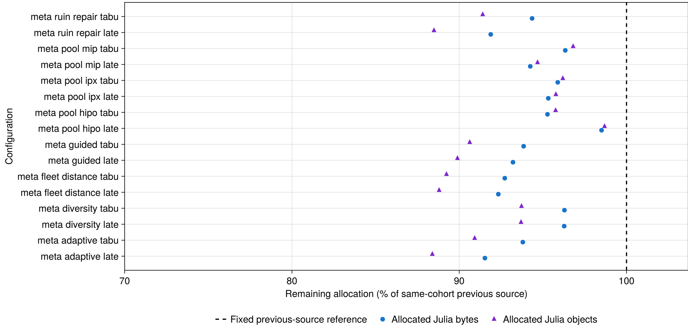
Routing meta profiles: independent primitive route snapshots
