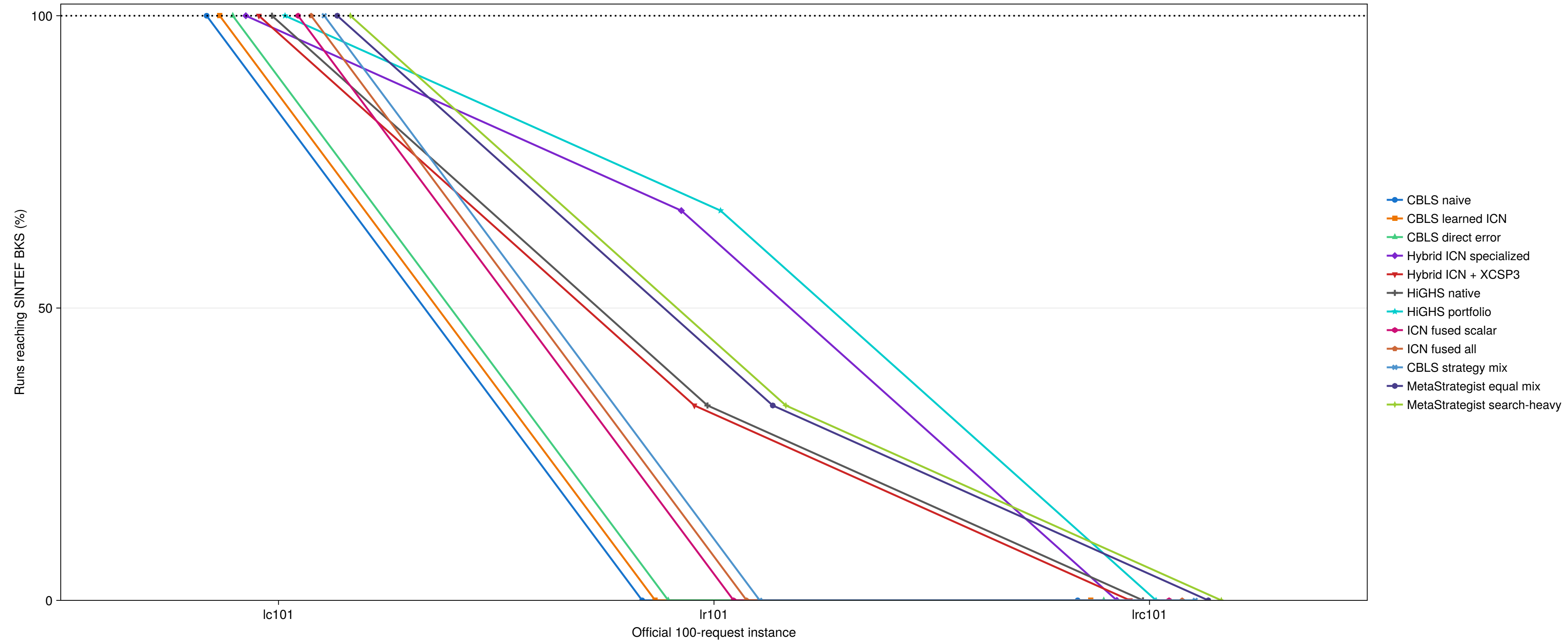
Best-Known Solution Success by Instance
