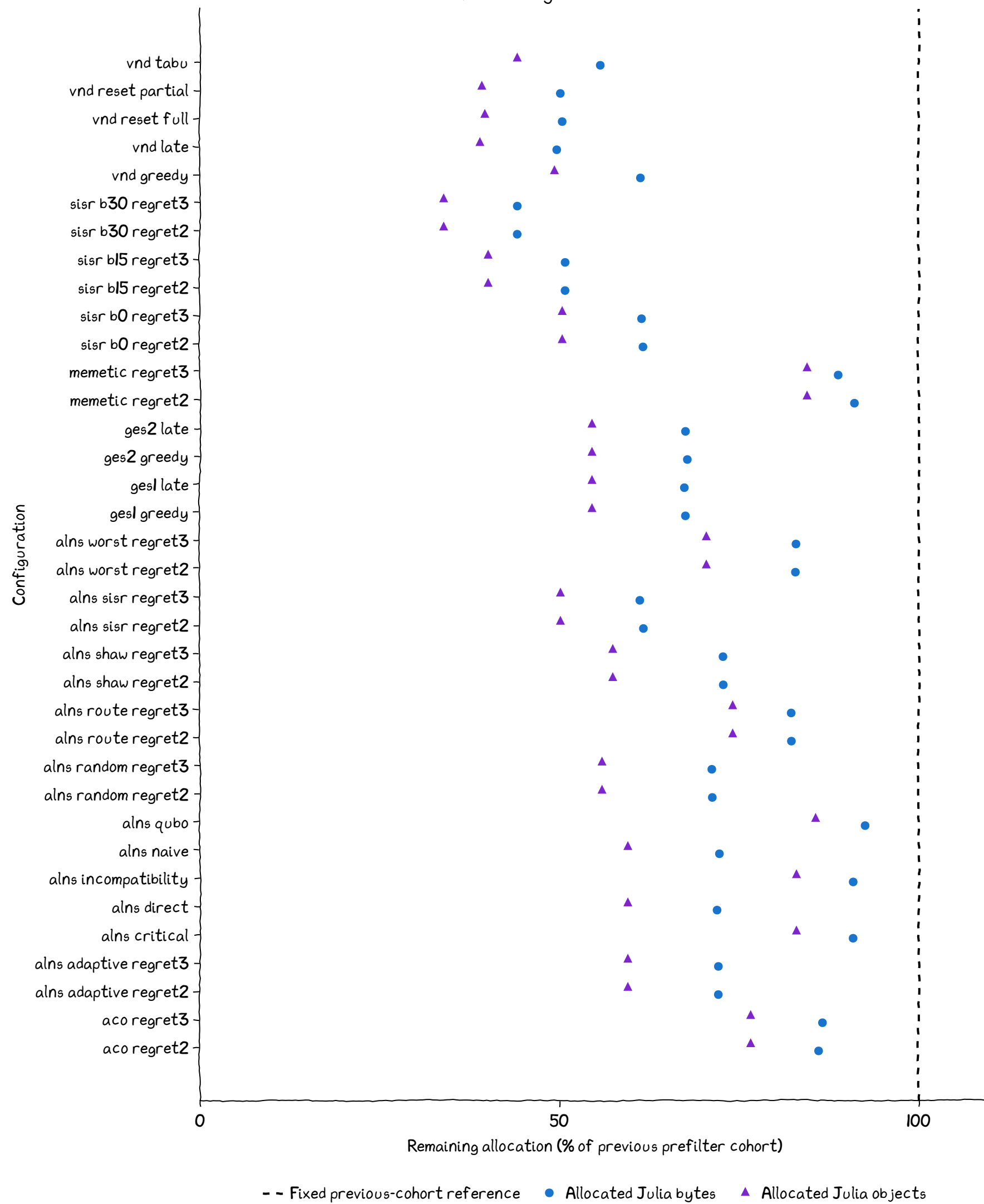
Fixed-work search configurations: additional allocation reduction
