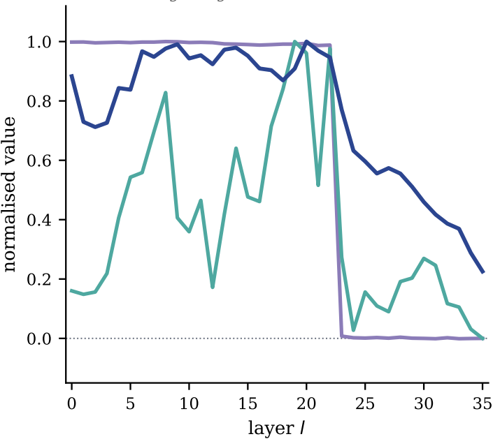
(a) Carry — ones b position
