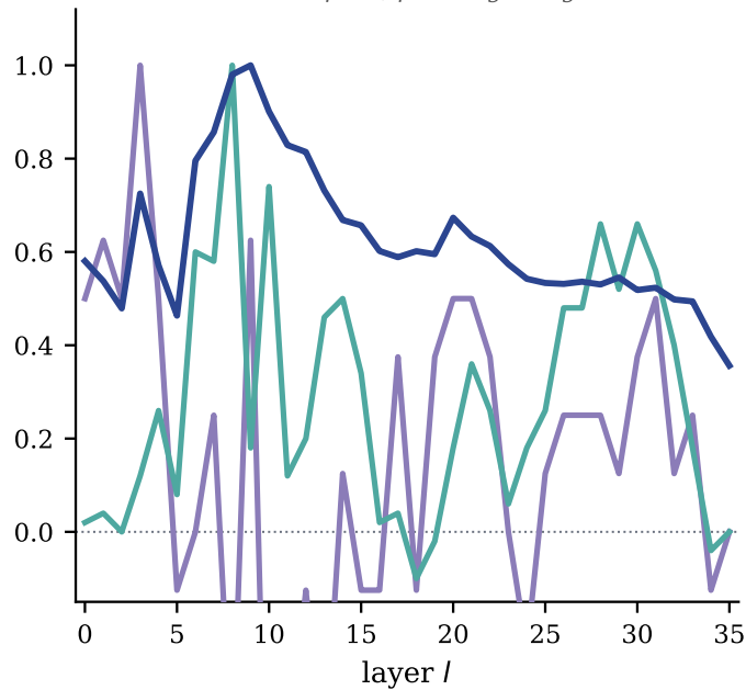
(b) Carry — operator position
