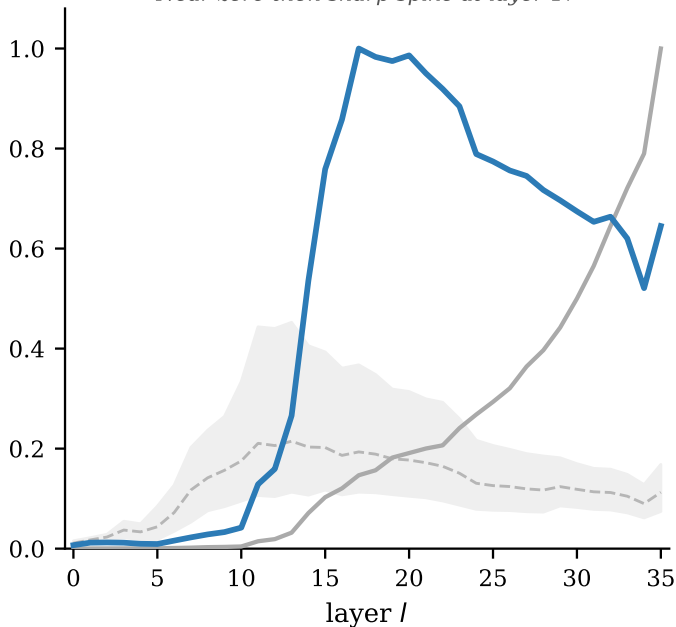
(b) GCD — operator position (pos 10)
