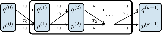
SympNet
