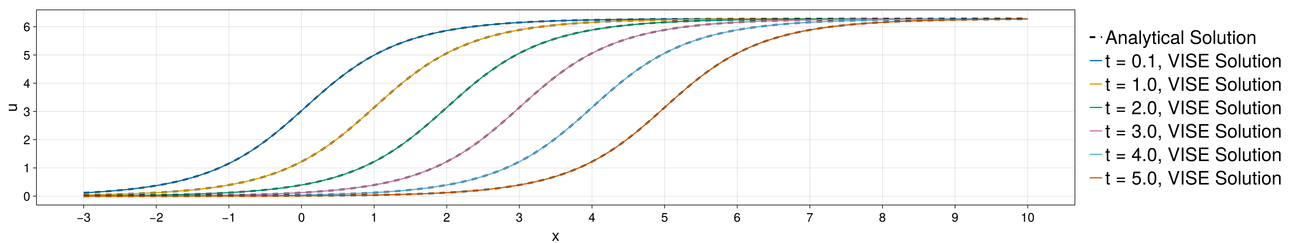
Sine-Gordon Equation
