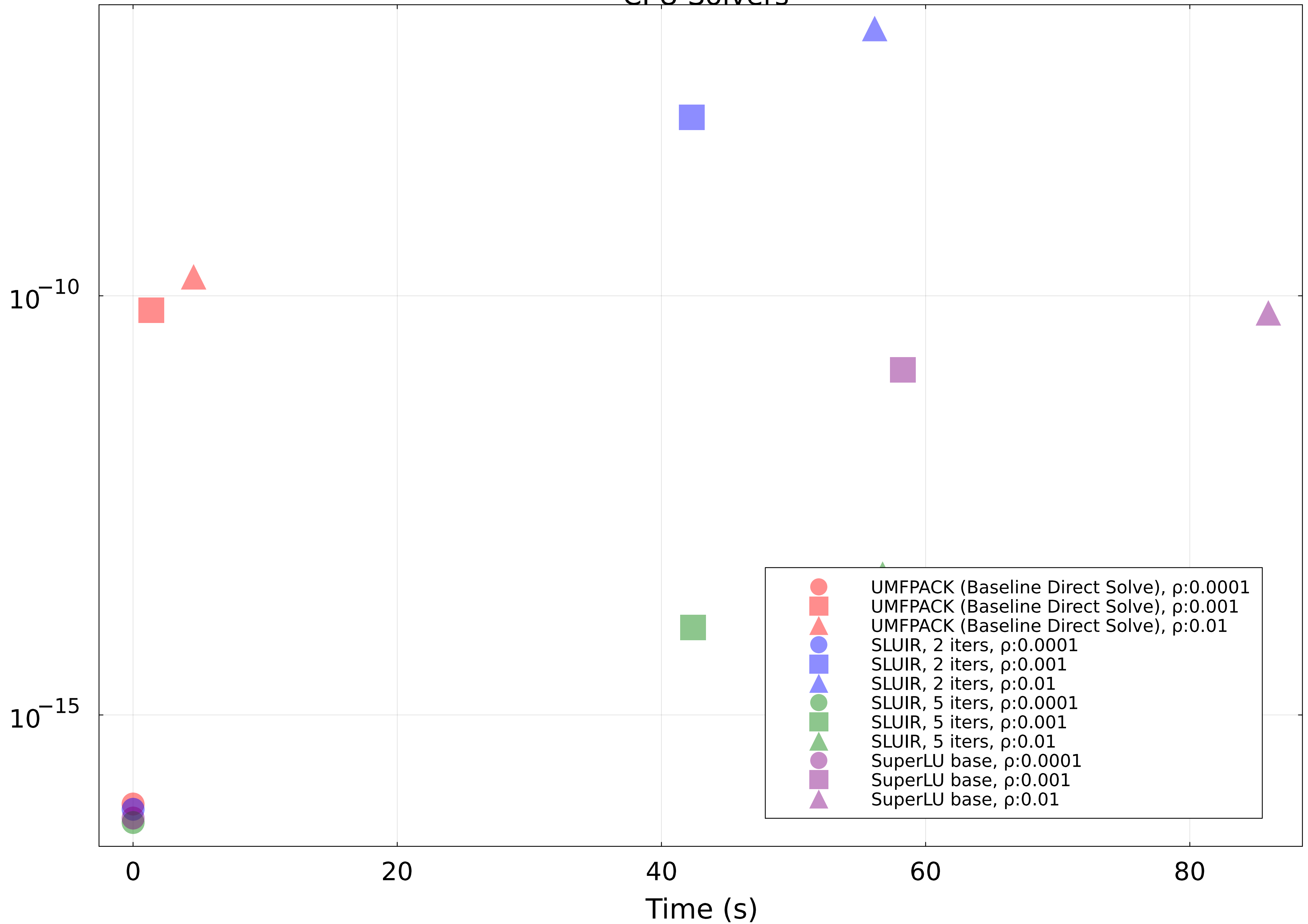
Random Matrices of Size 10000x10000, Varying Sparsity Levels ( \rho ) and CPU Solvers
