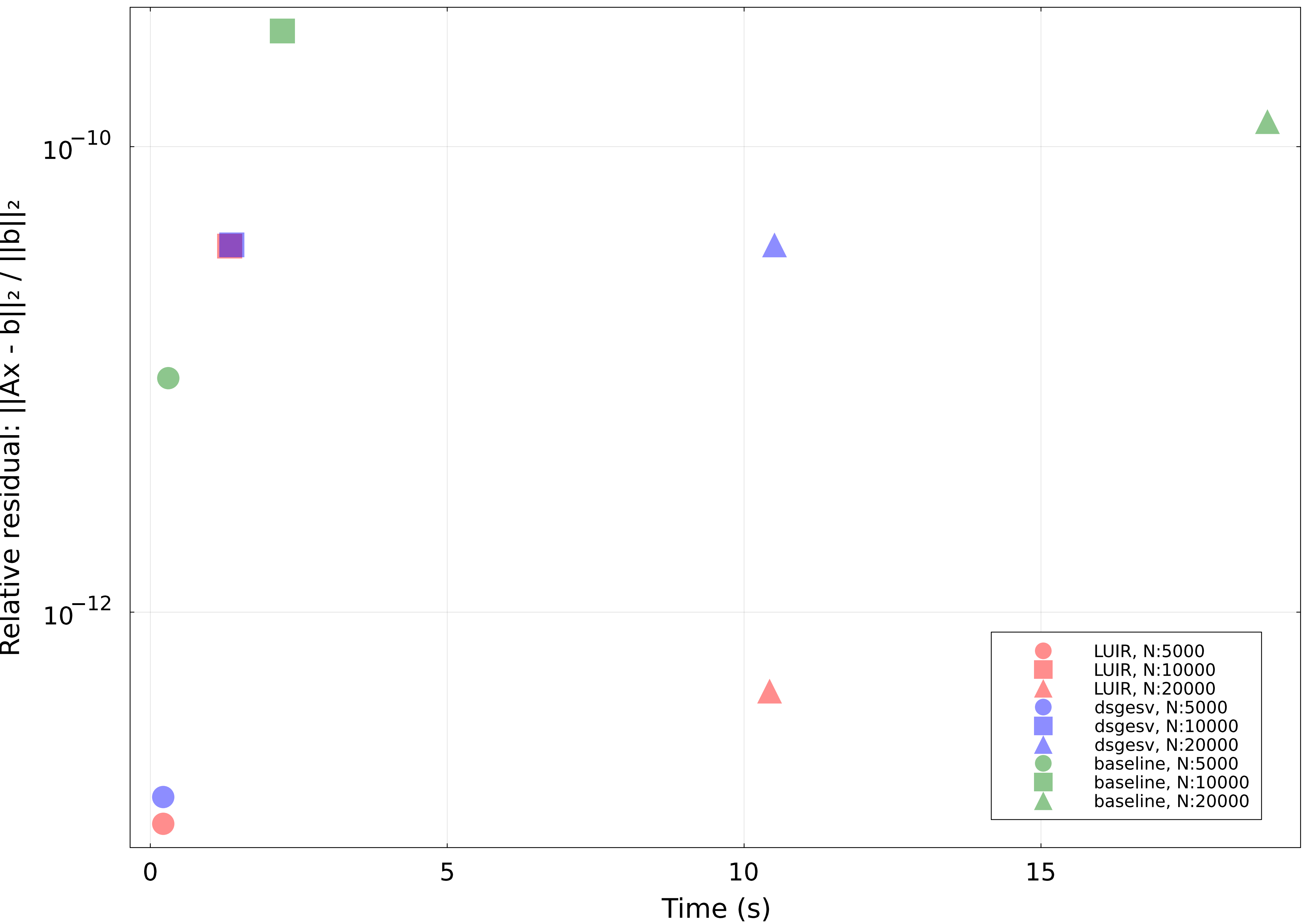
Dense Random Matrices of Varying Size (N) and CPU Solvers
