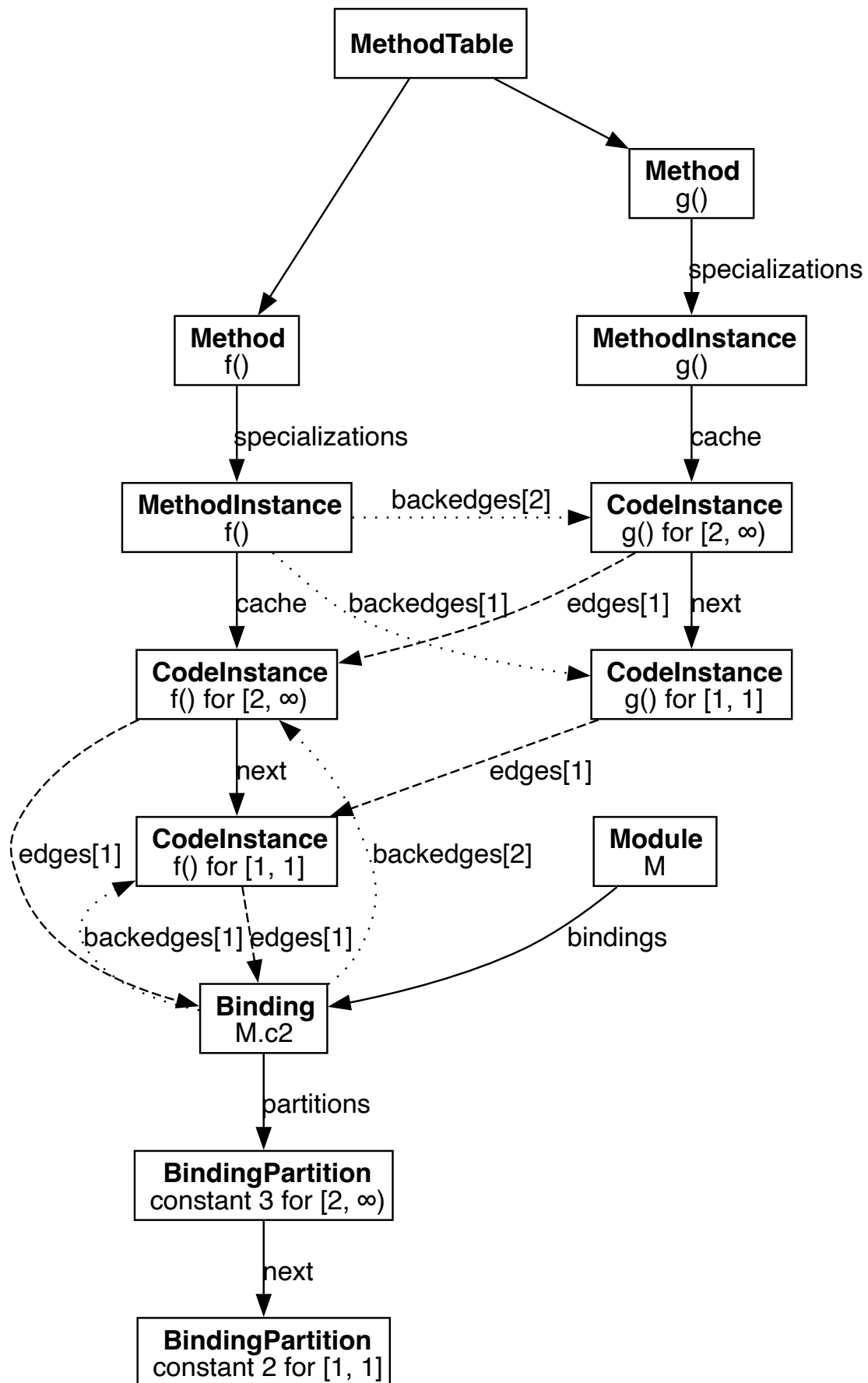
Figure 109.2: Global cache state after invalidation
