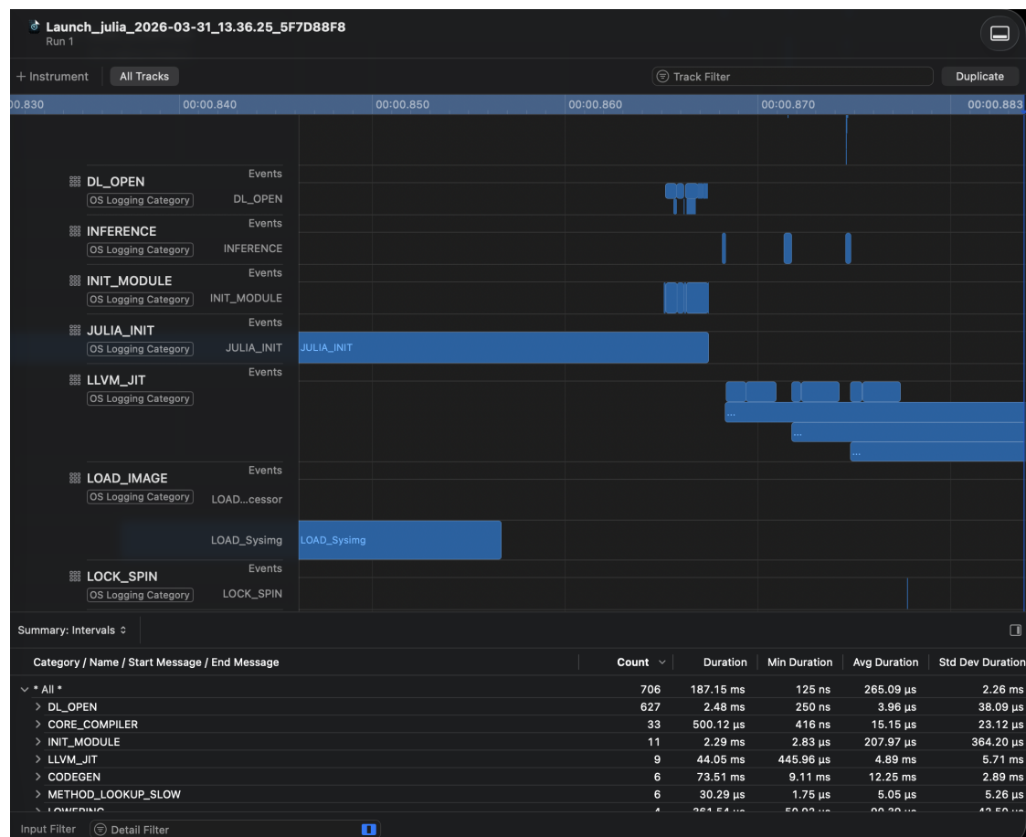
Figure 110.2: Typical Instruments usage
