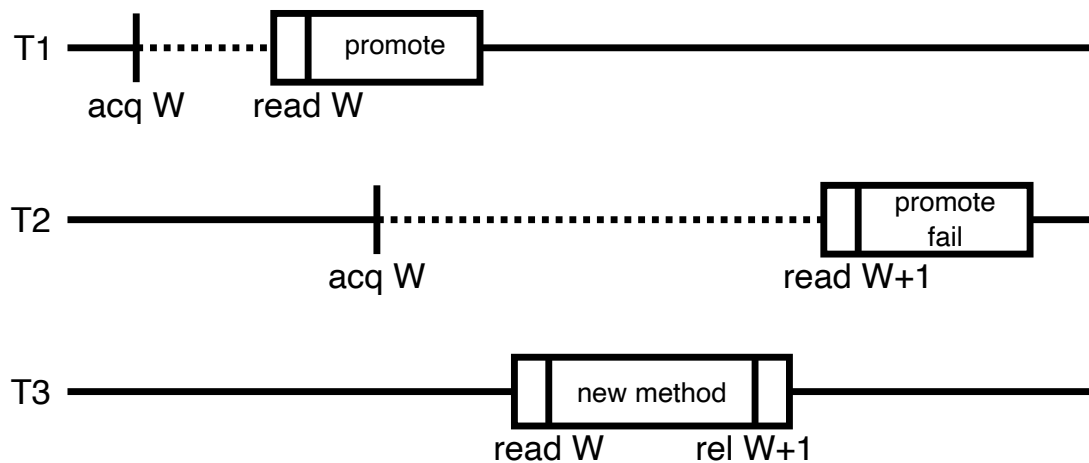
Figure 109.3: Two threads doing type inference while another adds a method
