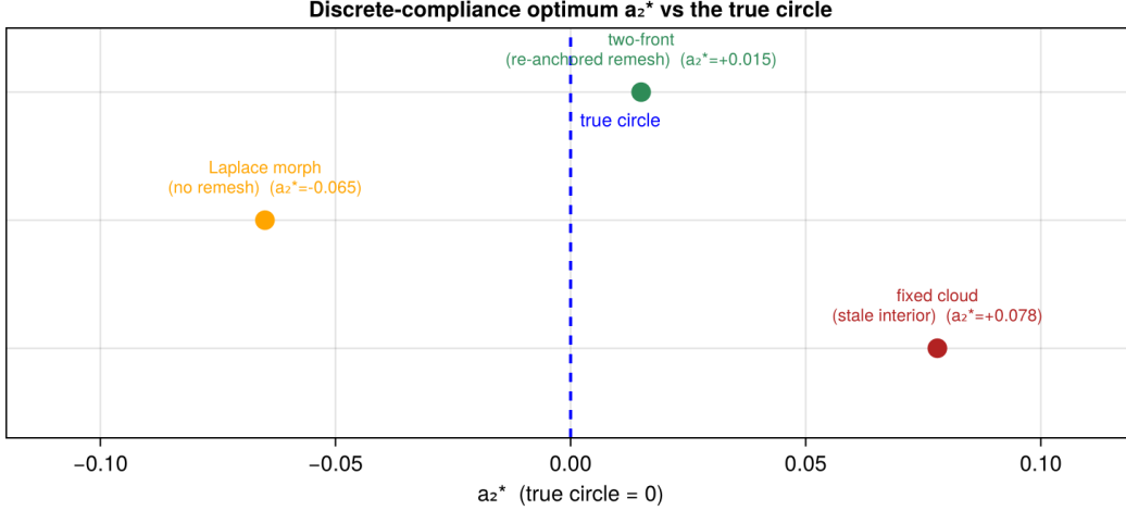
Figure 6: The objective bias is a stale-cloud artifact, not intrinsic. The discrete-compliance optimum a_2^* is displaced from the true circle ( a_2=0 ) and the sign brackets : a frozen interior gives +0.078 , a Laplace-morphed interior -0.065 . Re-anchored re-meshing (two-front) lands at +0.015 — essentially the circle.
