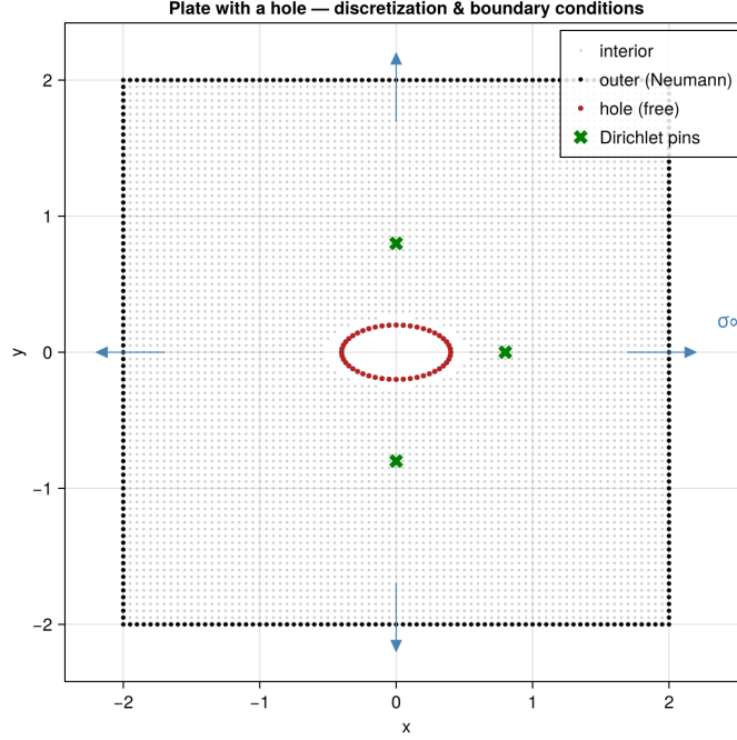
Figure 4: The plate-with-hole discretization: the interior cloud, the outer Neumann frame under biaxial traction \sigma_\infty , the free (traction-free) hole boundary, and the three Dirichlet pins that remove rigid-body modes.
