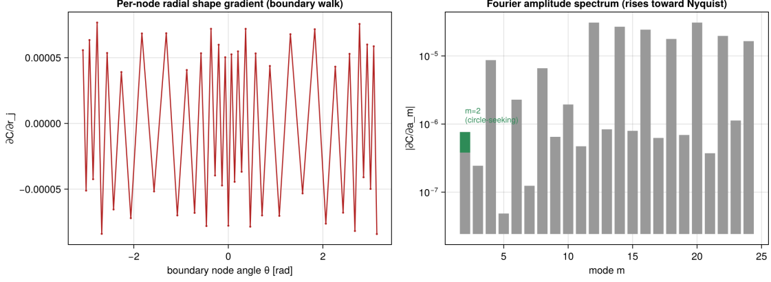
Figure 5: The boundary gradient noise. Left : the per-node radial shape gradient \partial C/\partial r_j walked around the hole — a near-Nyquist sawtooth. Right : its Fourier amplitude spectrum rises toward the highest representable mode; the circle-seeking m=2 mode (green) sits far below the high-mode band. The gradient is FD-exact yet genuinely rough.
