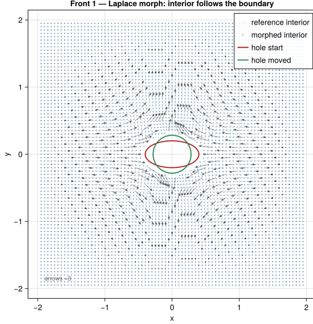
Figure 7: Front 1 (morph). As the hole moves from the start ellipse (red) toward the circle (green), the differentiable Laplace extension carries the interior nodes inward (displacement arrows, \times 3 ), decaying smoothly with distance. The adjoint flows back through this map by its transpose.
