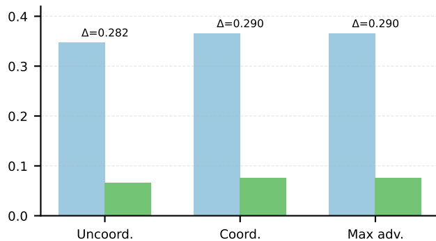
Qwen2.5 7B: centroid shift
