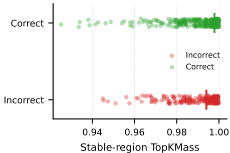
TopKMass vs. correctness
