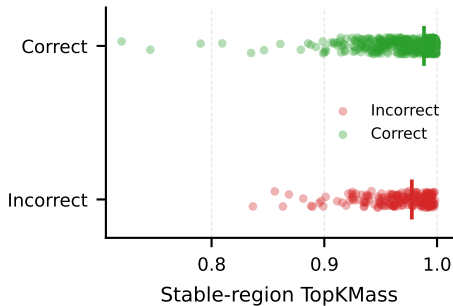
TopKMass vs. correctness
