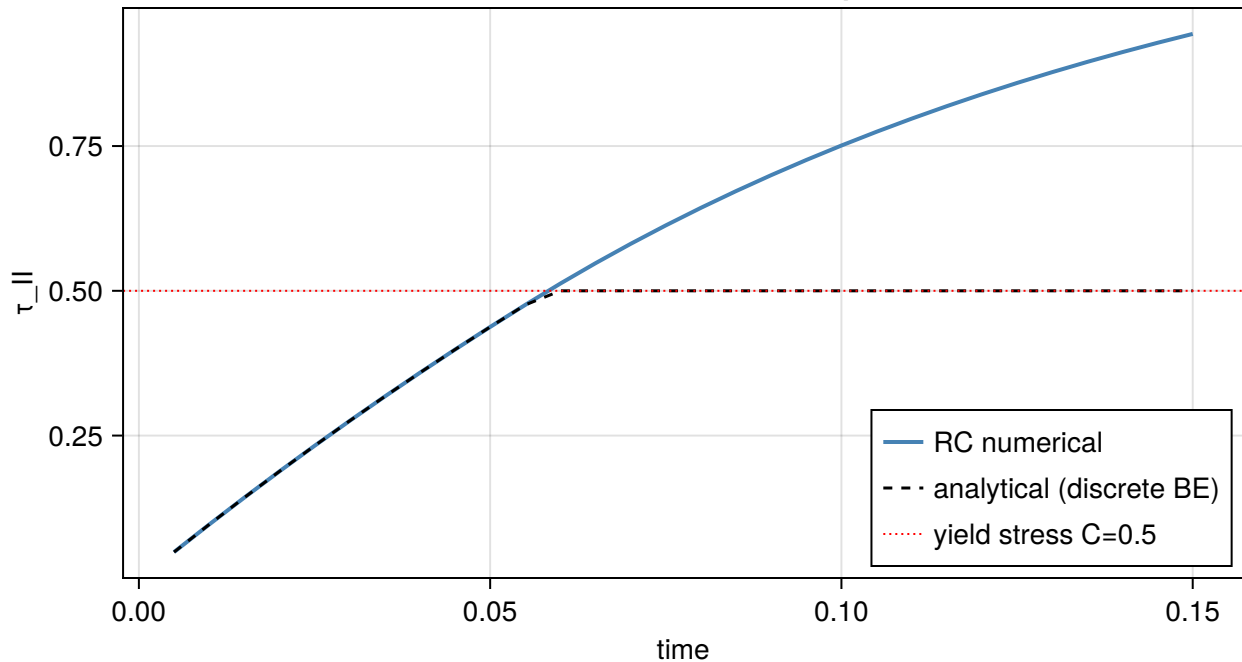
0D Maxwell VEP ( \eta=1.0 , G=5.0 , C=0.5 , \eta_{vp}=0.001 , dt=0.005 )
