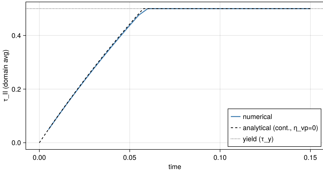
Maxwell VEP stress build-up
