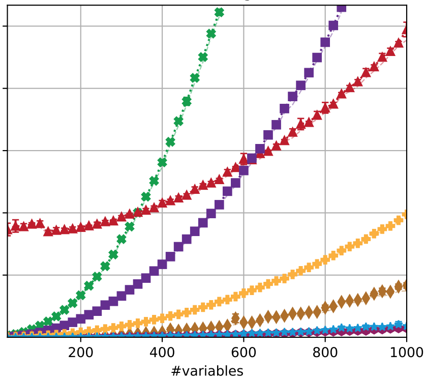
Number Partitioning Problem
