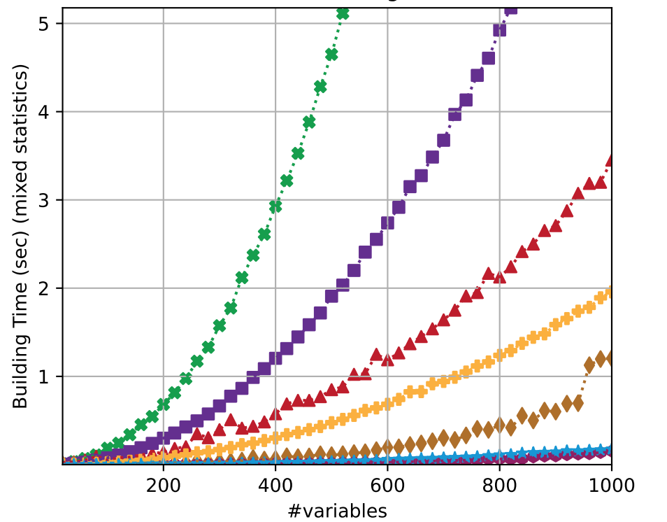
Number Partitioning Problem
