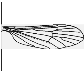
Tipulidae wing
