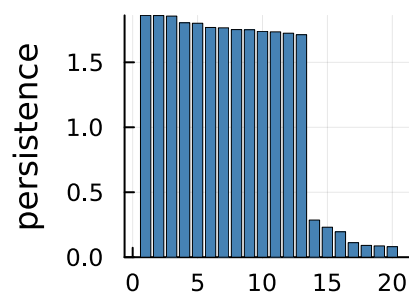
Radial H0
