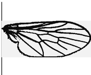
Rhagionidae wing
