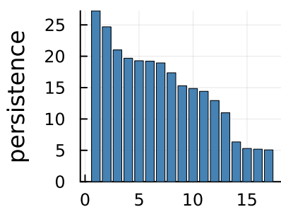
Rips H1
