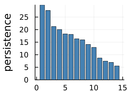
Rips H1
