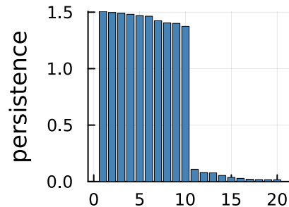
Radial H0
