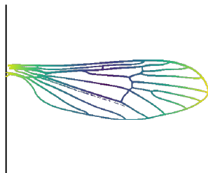
T-19 radial
