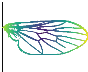
R-10 radial
